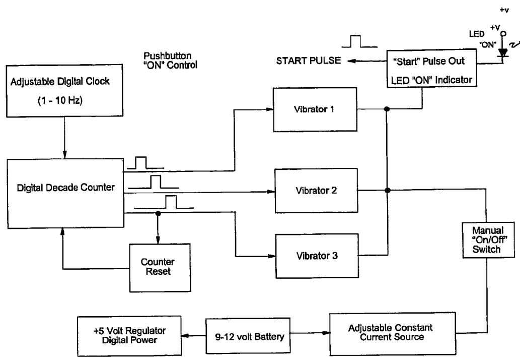
BLOCK DIAGRAM VIBRO-TACTILE STIMULATOR NTM 6/27/2006
