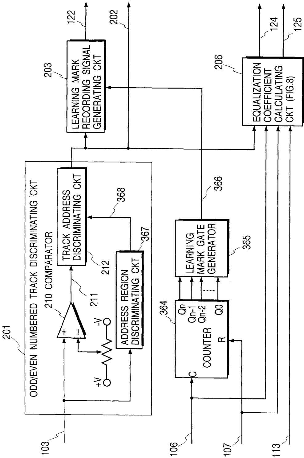
121 EQUALIZATION COEFFICIENT LEARNING CKT
