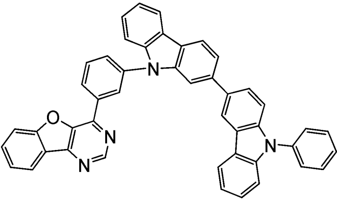
4mPCCzPBfpm-02
