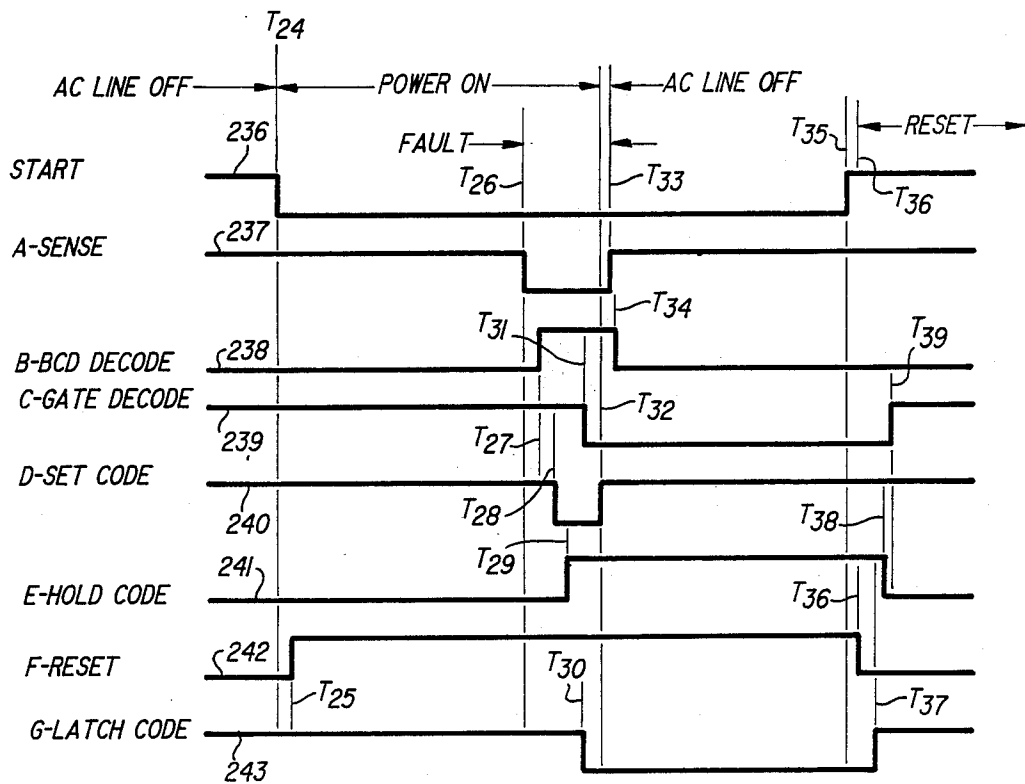
FIG. 8 FAULT CODE RETENTION
