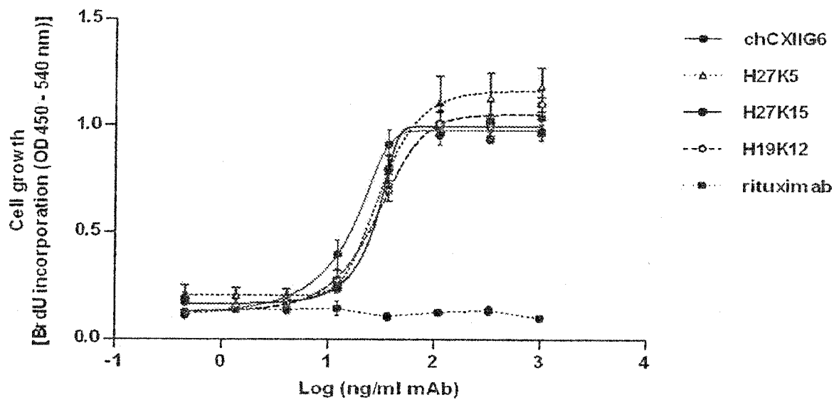
Fig. 28 : Blockade of soluble CD115 by hCXIIIG6 variants and chCXIIIG6 in the M-NFS-60-cell based assay
