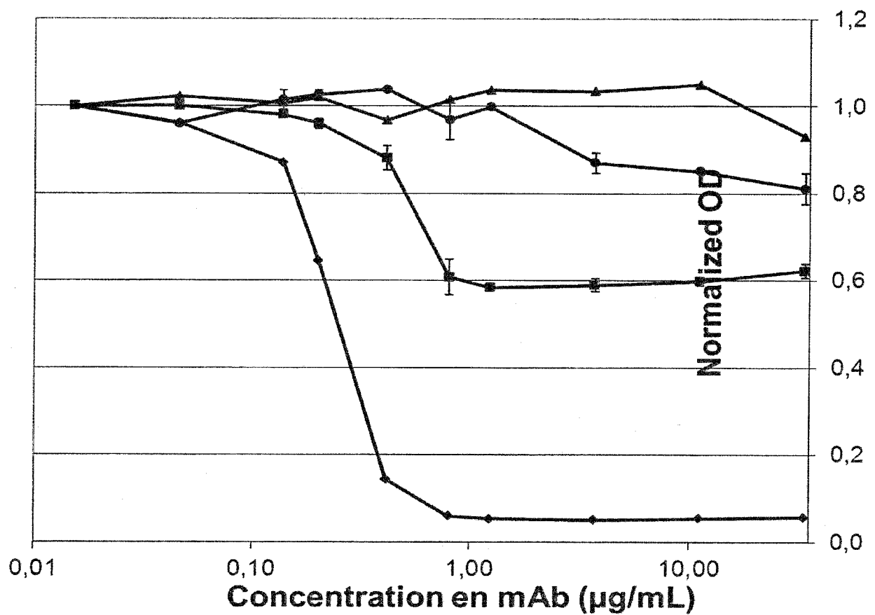
Fig. 24 :Preincubation competition: mAb (1hour), then CSF1-biot (1hour)
