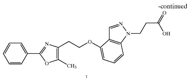
3-{4-[2-(5-methyl-2-phenyl-1,3-oxazol-4-yl)ethoxy]-1H-indazol-1-yl}propanoic acid
