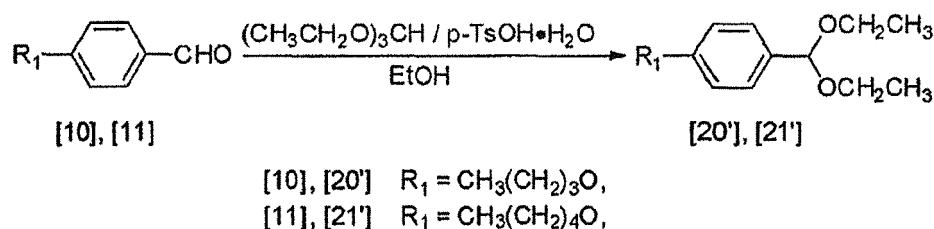
Scheme 4
