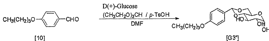
Scheme 10
