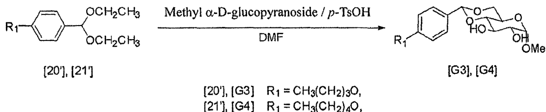
Scheme 7
