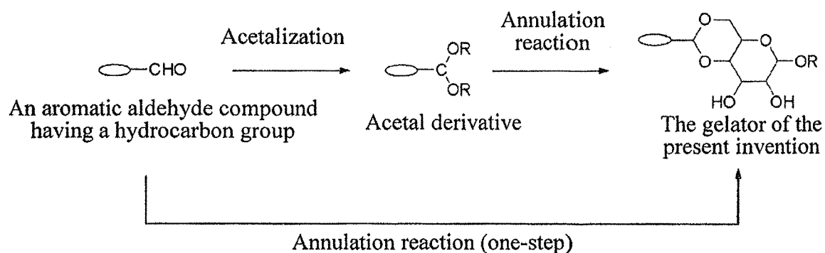
Scheme A: Synthetic routes of one-step reaction and two-step reaction
