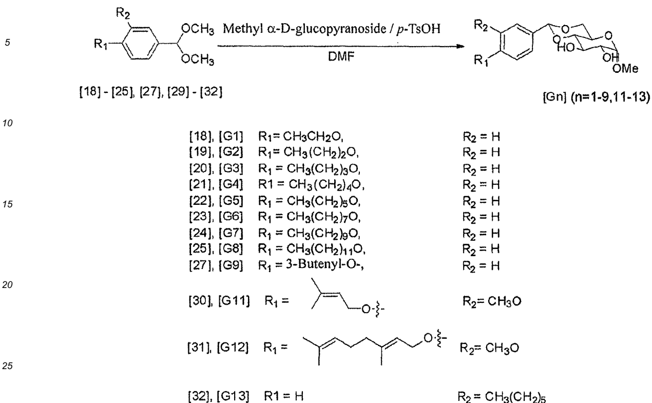
Scheme 6
