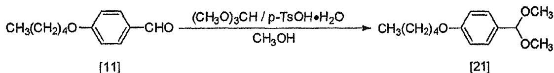
Scheme 3
