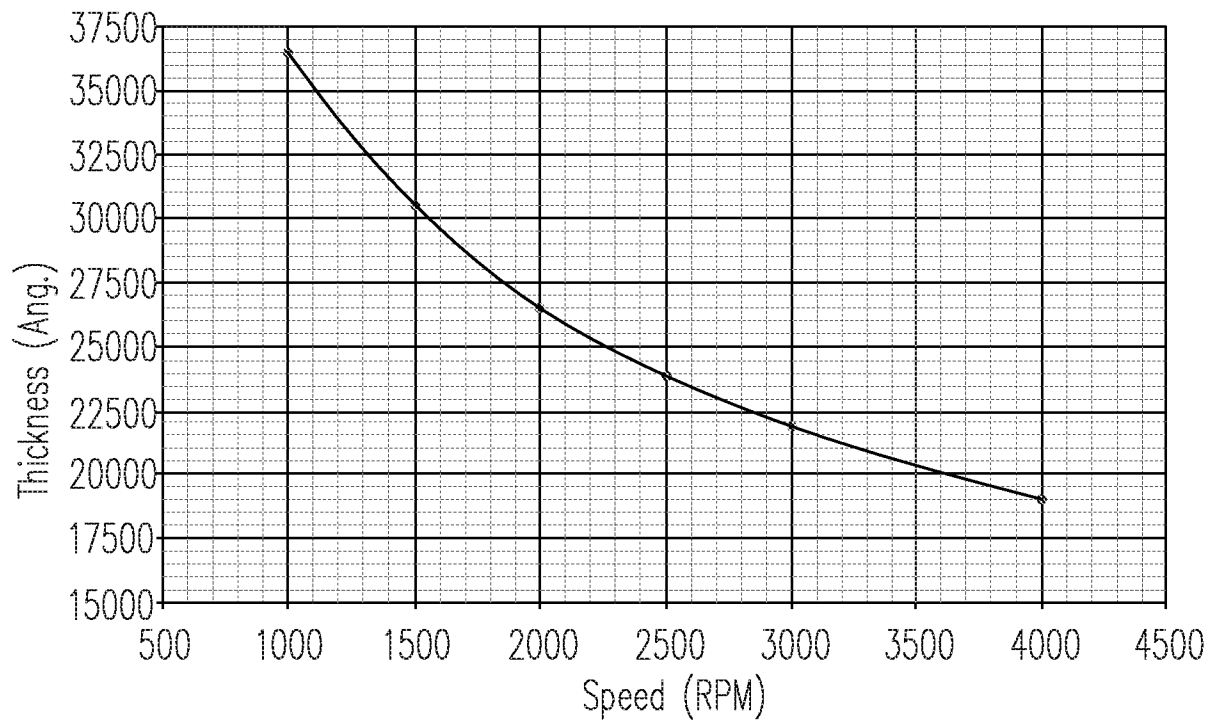
GRAPH 1: An Illustration of Thickness of the First Dielectric Material Versus the Spin Rate (i.e., Speed) of the Semiconductor Material
