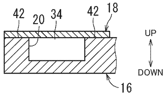
CROSS-SECTIONAL VIEW TAKEN ALONG LINE V-V
