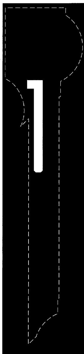
N-Well mask
