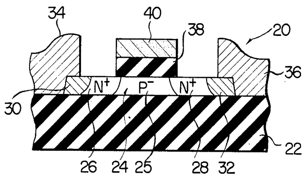
FIG. 1 (PRIOR ART)
