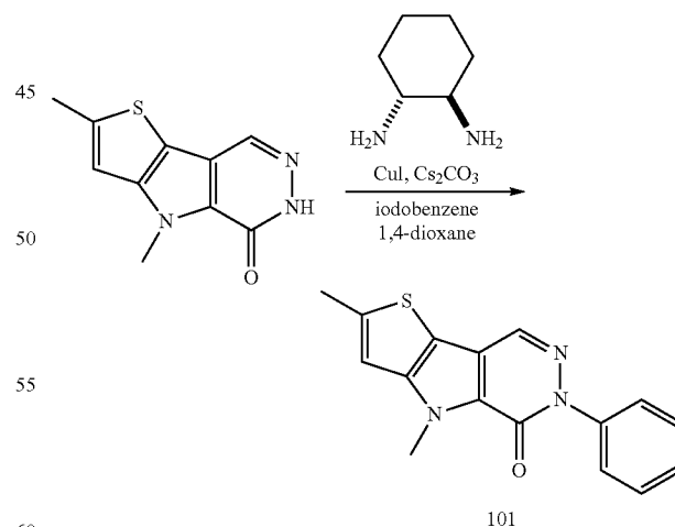
2,4-Methyl-6-[(2-fluorophenyl)methyl]-4H-thieno[3,2-b]pyrrole[3,2-d]pyrimidinone (101)
