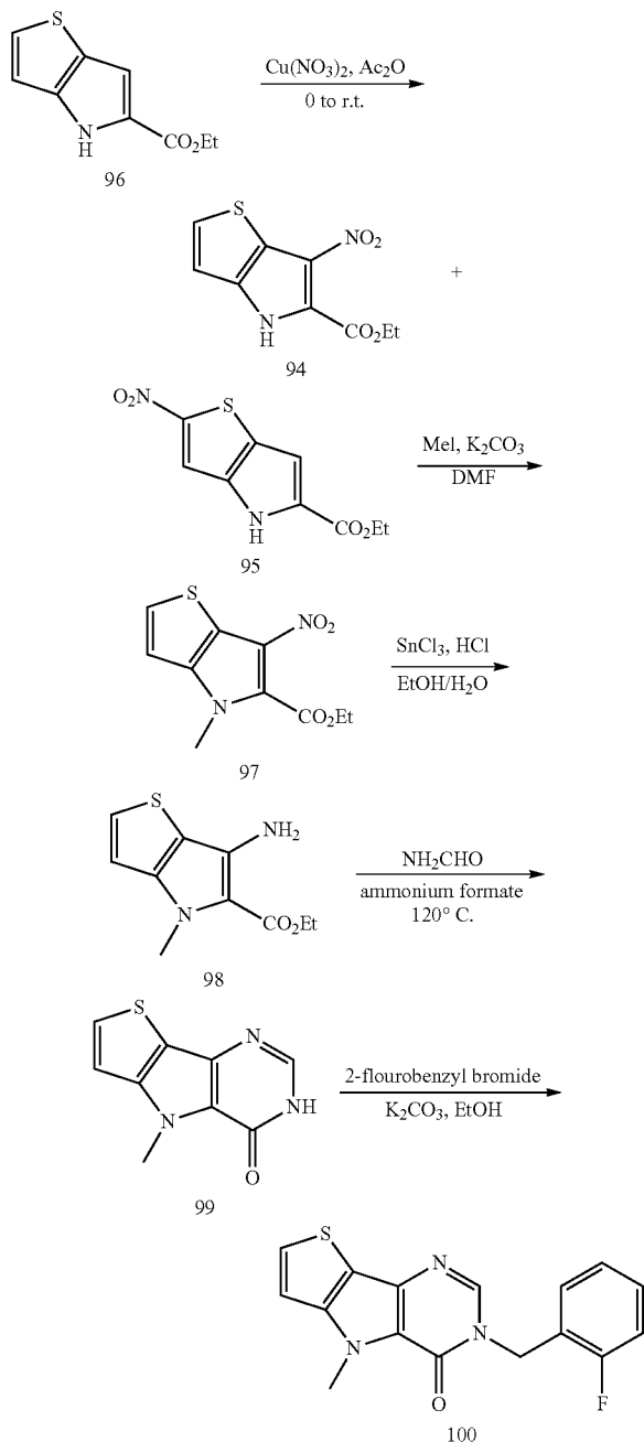
Ethyl-6-amino-4-methyl-4H-thieno[3,2-b]pyrrole-5-carboxylate (98)
