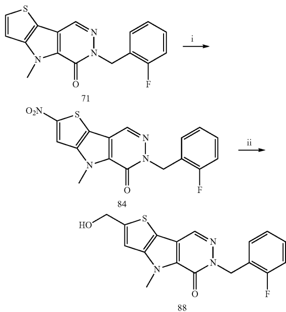
Scheme 7
