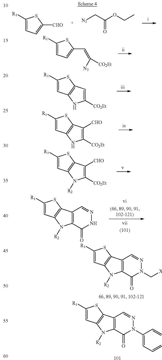
Scheme 4
