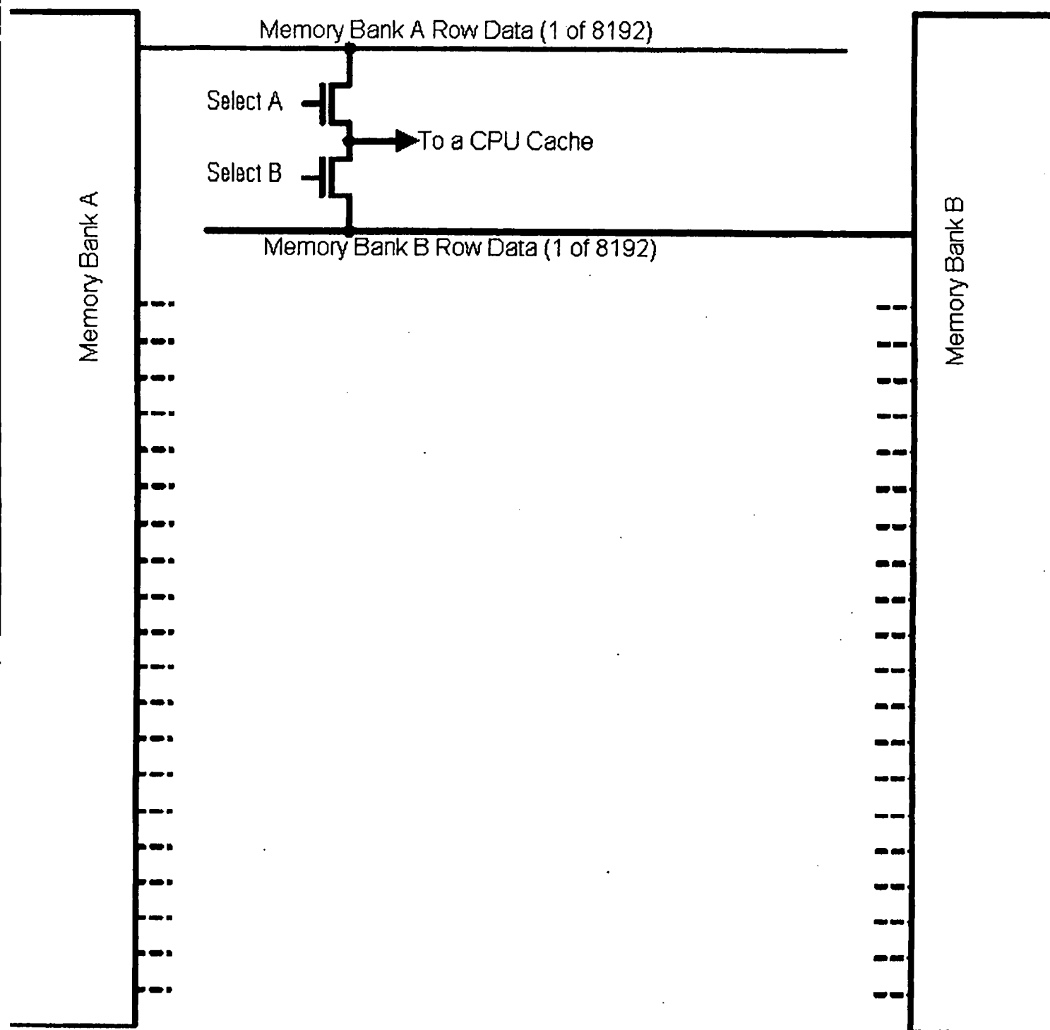
Sharing Memory Banks Fig. 7B
