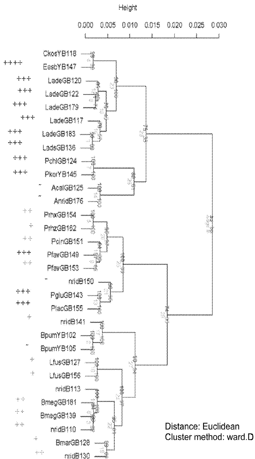
Cluster dendrogram with AU/BP values %
