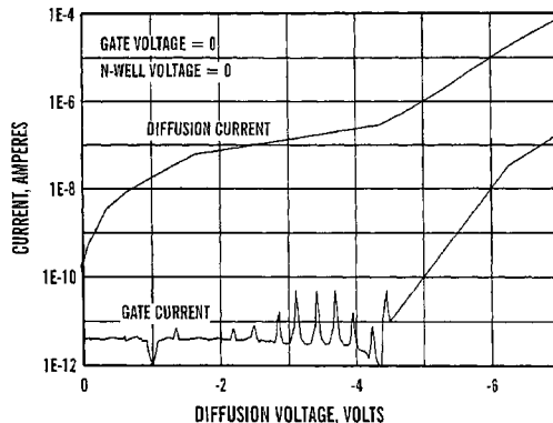
GATE AND DIFFUSION CURRENTS AT 180C AND 5nm THERMAL OXIDE
