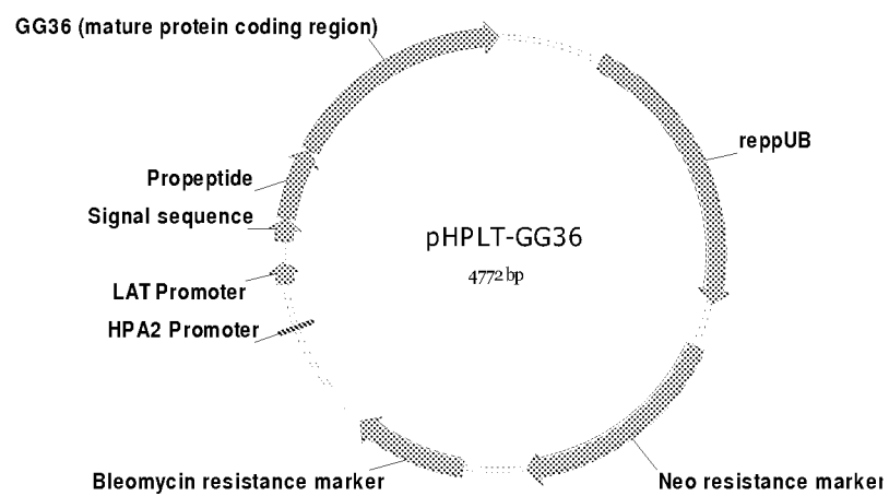
FIGURE 2 - pHPLT-GG36 Expression Plasmid
