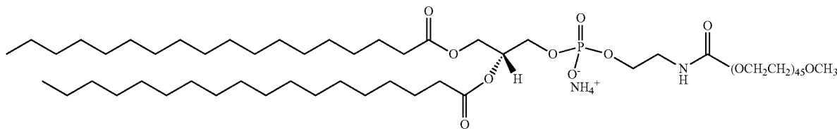
DSPE-PEG2000
