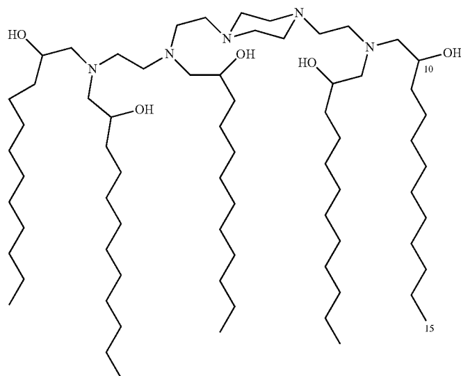
DLin-MC3-DMA
