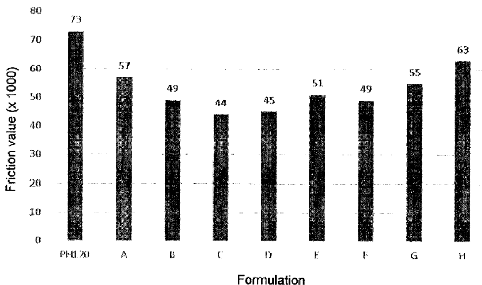
Friction values of the compositions A – H and the reference PH120
