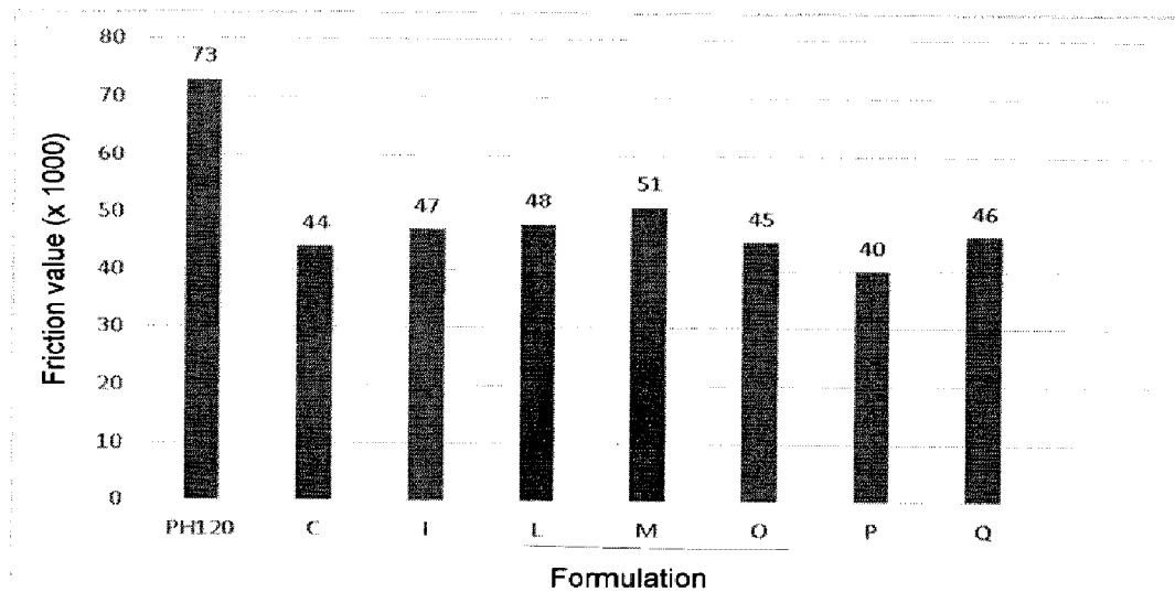
Fig. 3: Friction values of the compositions C, I, L, M, O, P, Q and the reference PH120
