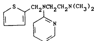
methapyrilene
