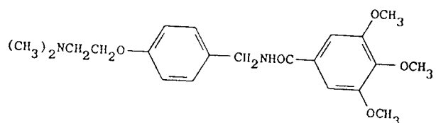
trimethobenzamide
