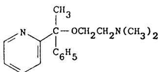
doxylamine
