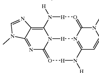
Reverse Watson Crick iGC-Base Pair VIII parallel
