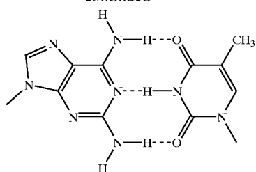
Watson Crick n 2 AT-Base Pair III antiparallel
