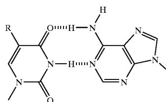
base pair IIa: R = H IIb: R = Br IIc: R = I
