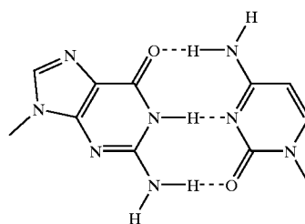
Watson Crick GC-Base Pair VII antiparallel
