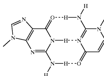
Reverse Watson Crick GiC-Base Pair IX parallel
