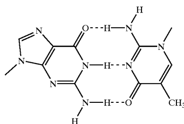
Reverse Watson Crick G mᵉ iC-Base Pair X parallel
