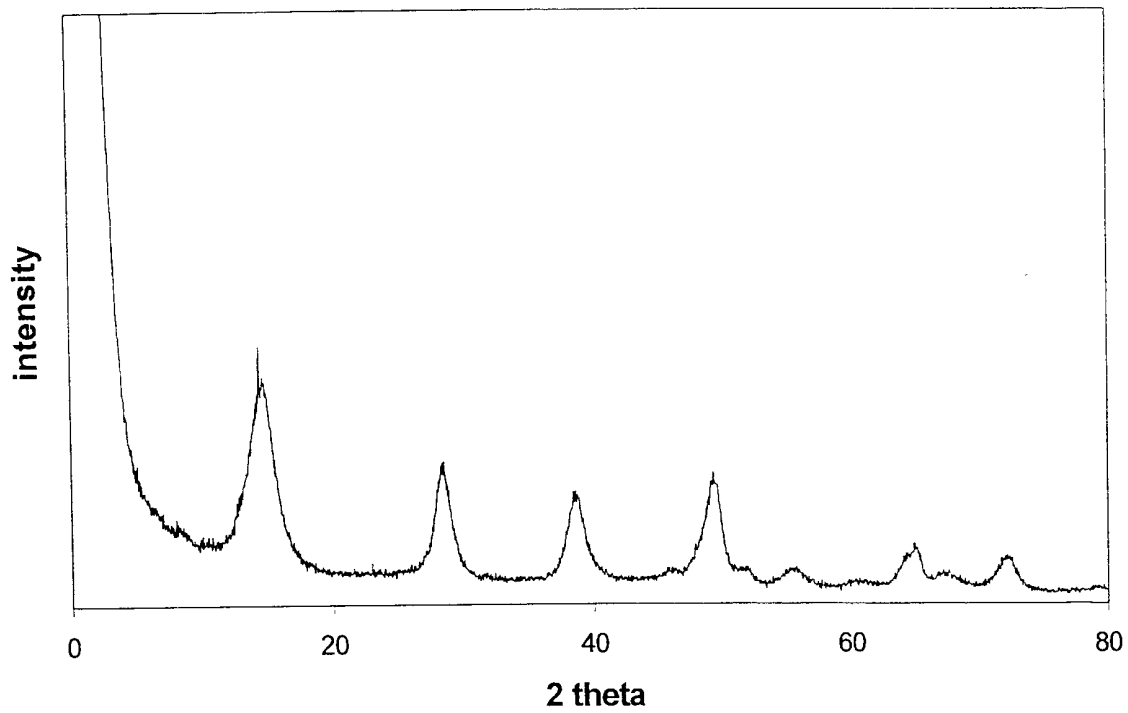
Figure 3 QCB prepared by hydrothermal treatment at pH=4
