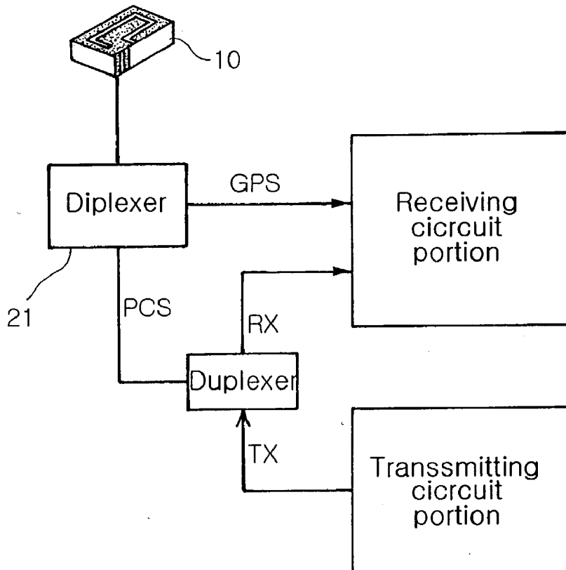
Prior Art FIG. 2b
