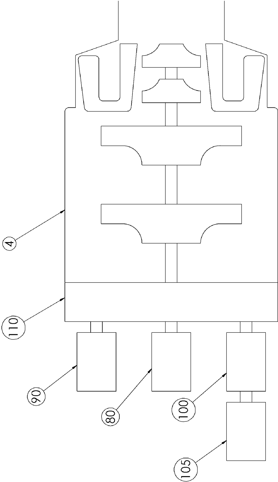
FIG. 2 (PRIOR ART)
