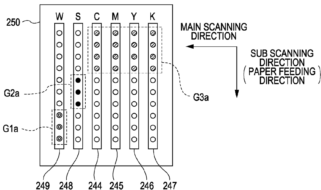
FIG. 6B SECOND PRINTING MODE
