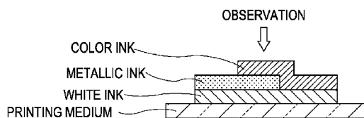
FIRST PRINTING MODE (PRINTING MEDIUM: LIGHT-TRANSMITTING PRINTING MEDIUM)
