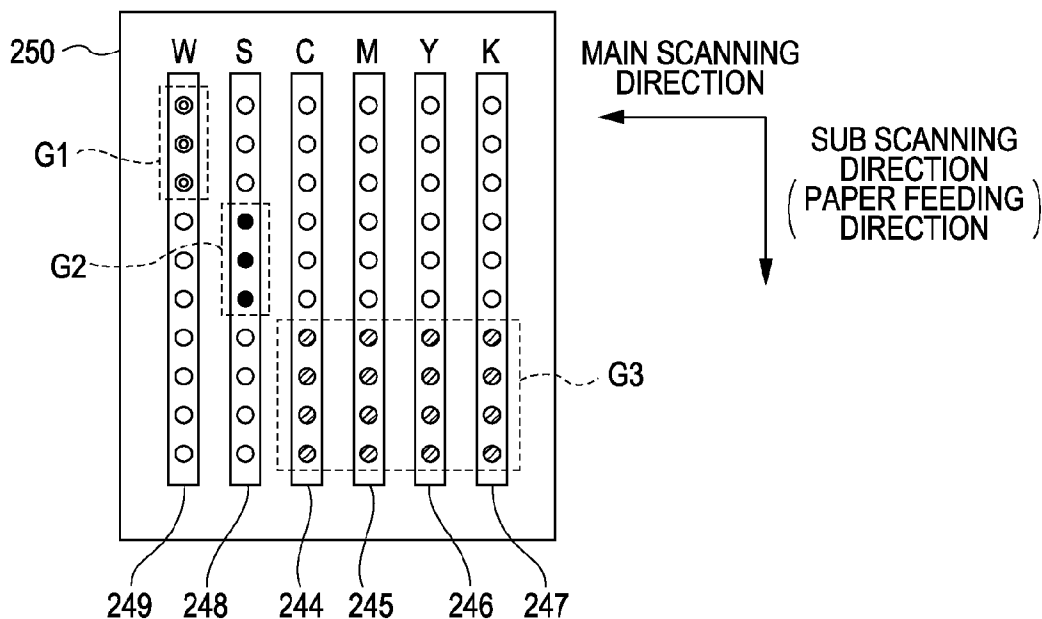
FIG. 6A FIRST AND THIRD PRINTING MODES
