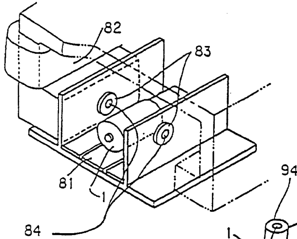
FIG. 10(b) LOCAL AC EXCITATION COIL-2
