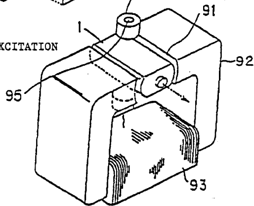
INDUCED MAGNETIC FIELD CHANGES DETECTING DEVICE
