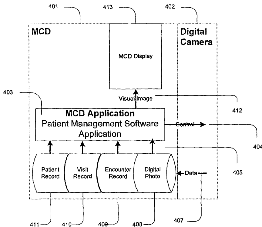
Mobile computing environment Components
