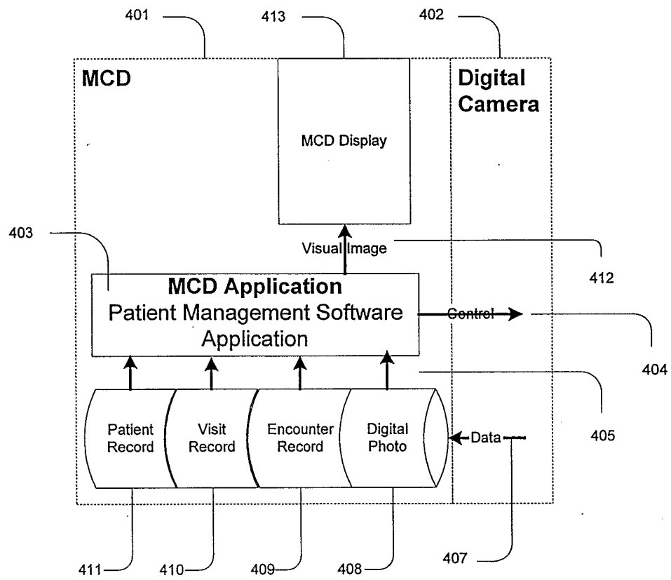
Figure 4 Mobile computing environment Components
