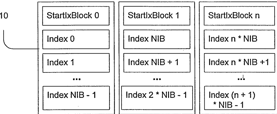
Figure 3 - Configuration Info and Indices
