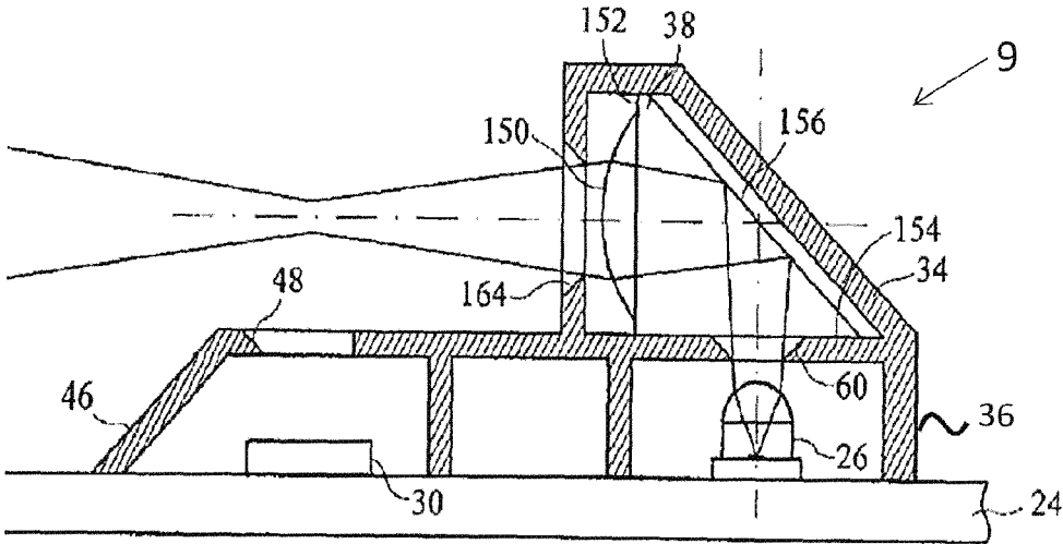
Figure 3 PRIOR ART
