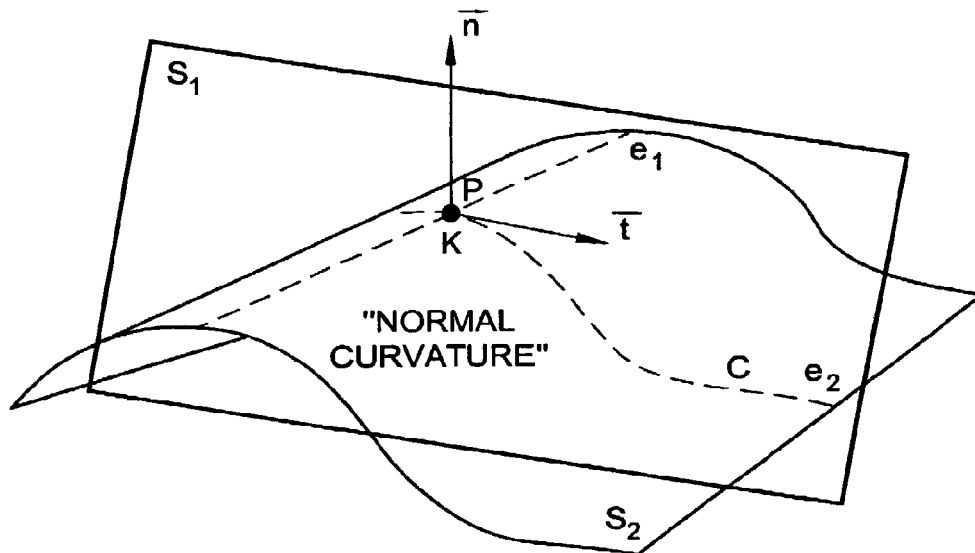
DIFFERENTIAL CHARACTERISTICS OF SURFACES
