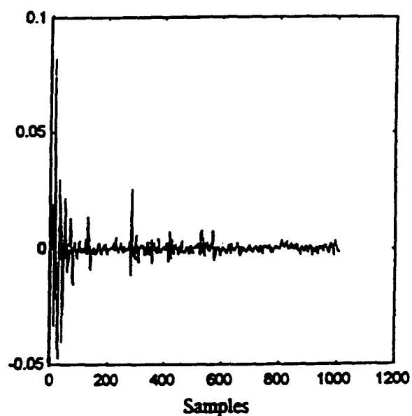
d) Right loudspeaker-right ear
