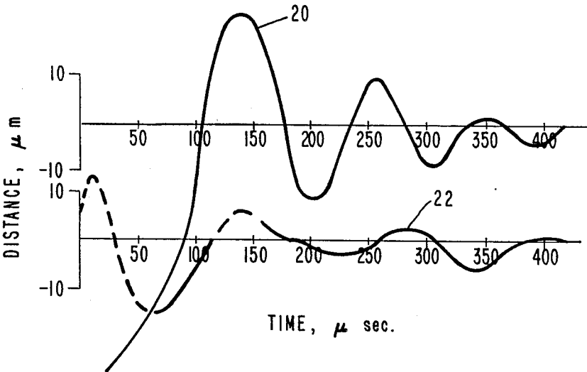
Fig. 2. (PRIOR ART)
