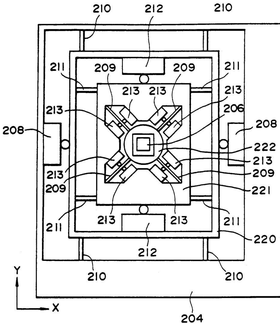
FIG. 9 PRIOR ART
