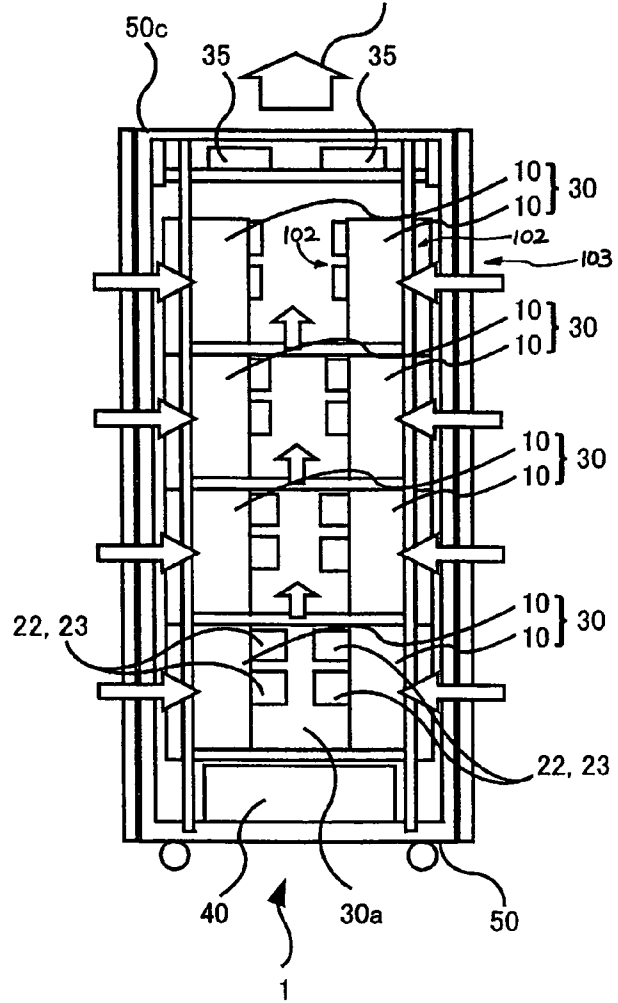
FIG. 1B AIRFLOW
