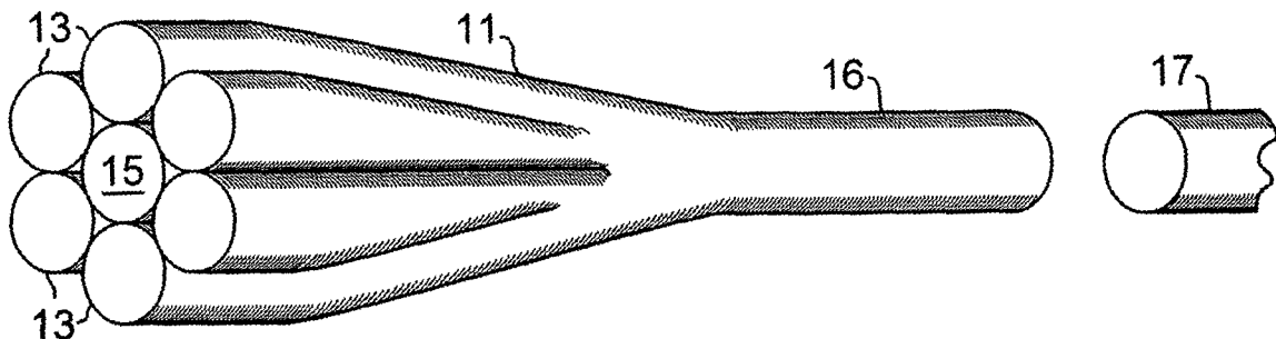
FIG. 1 (prior art)
