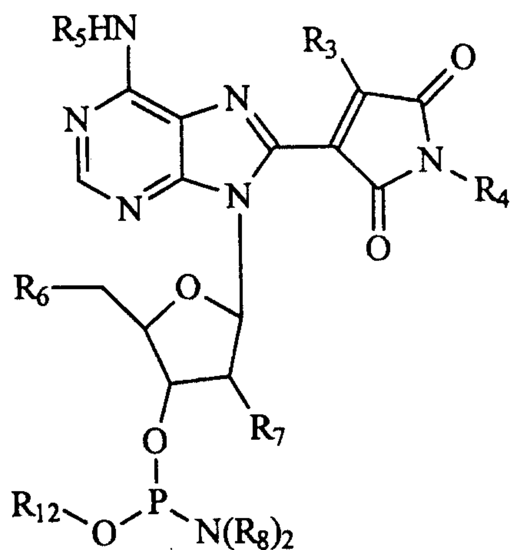
Structure X
