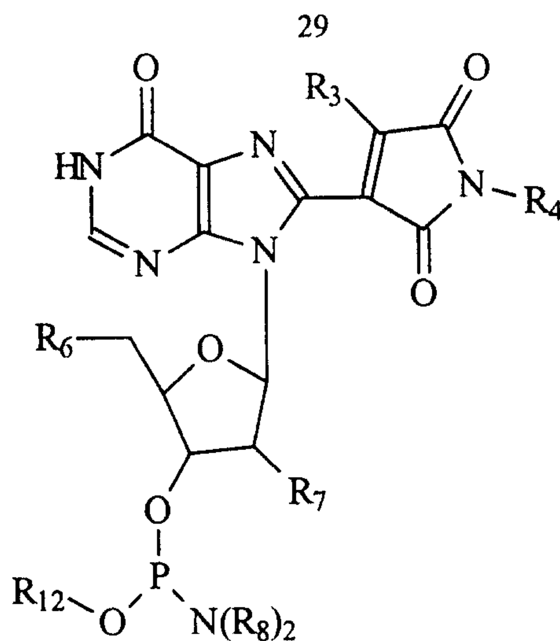
Structure Z
