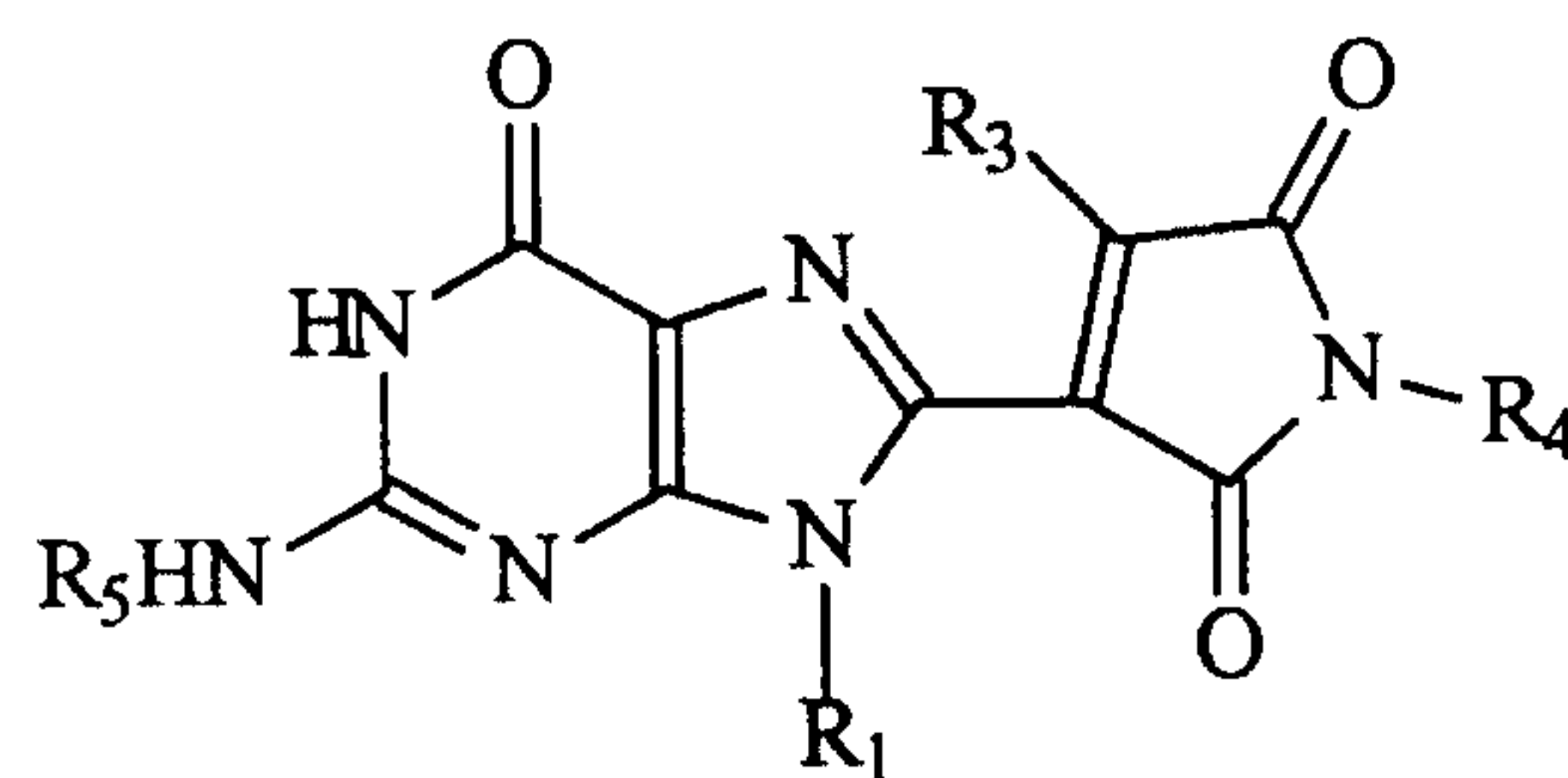
Structure T
