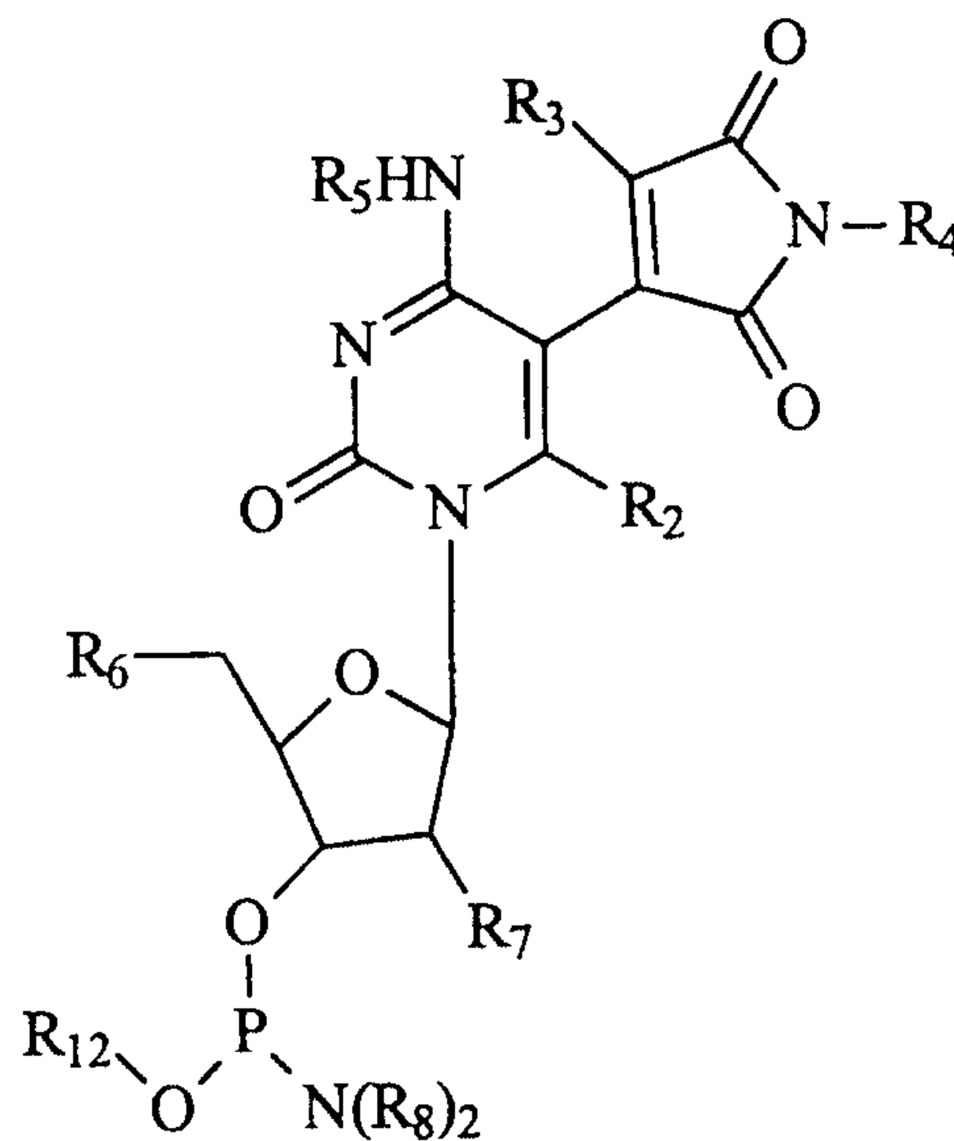
Structure W
