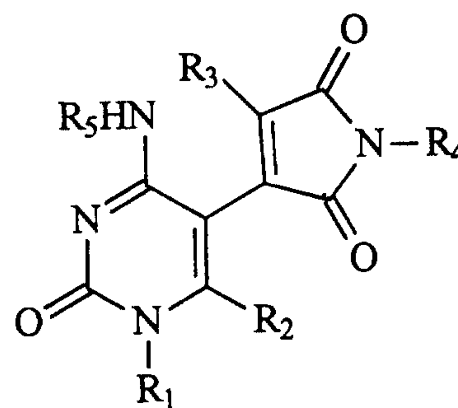
Structure R
