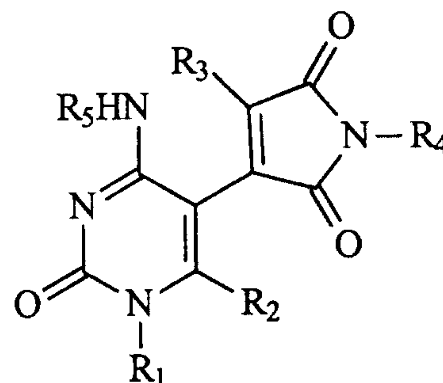
Structure R
