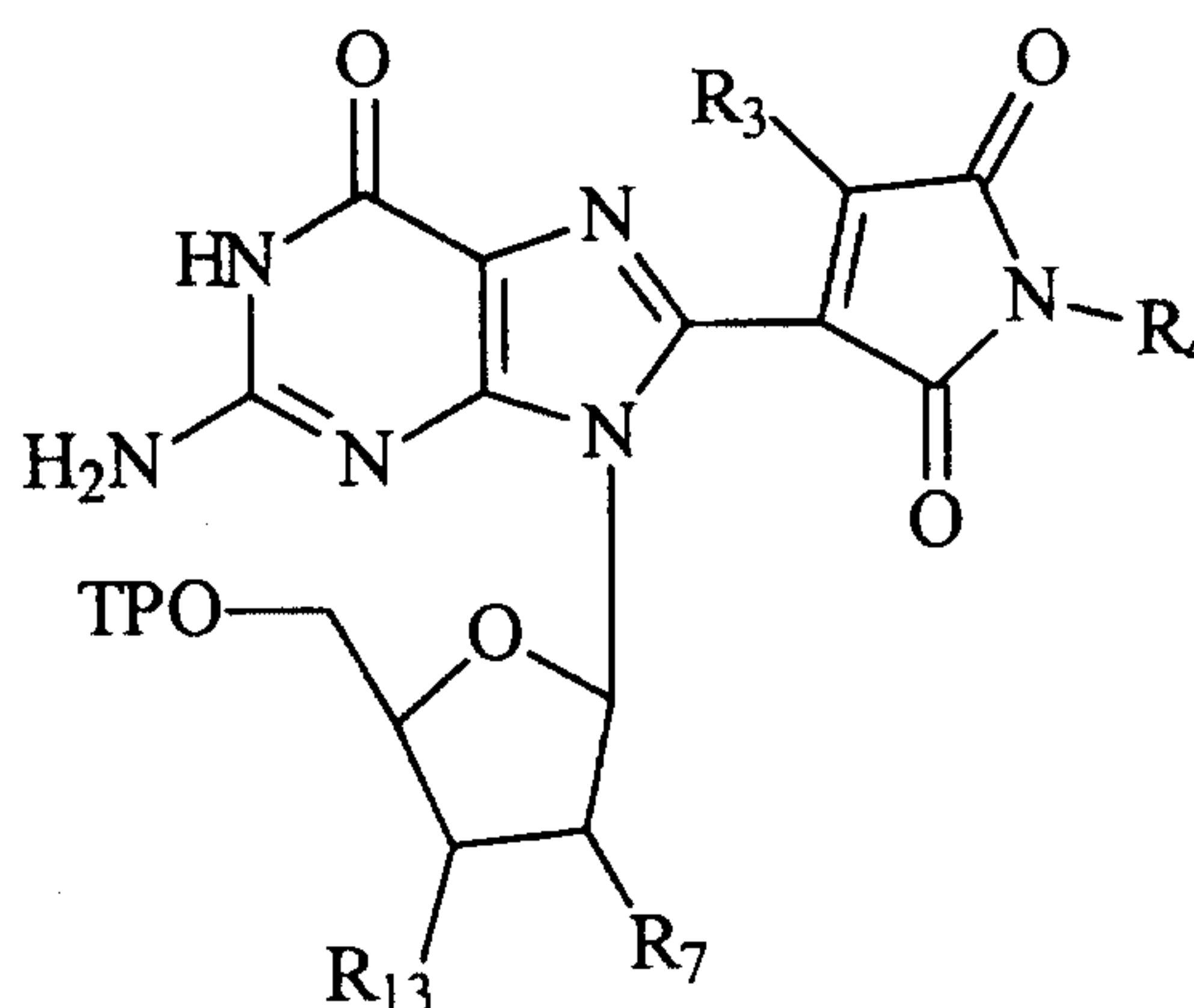
Structure I
