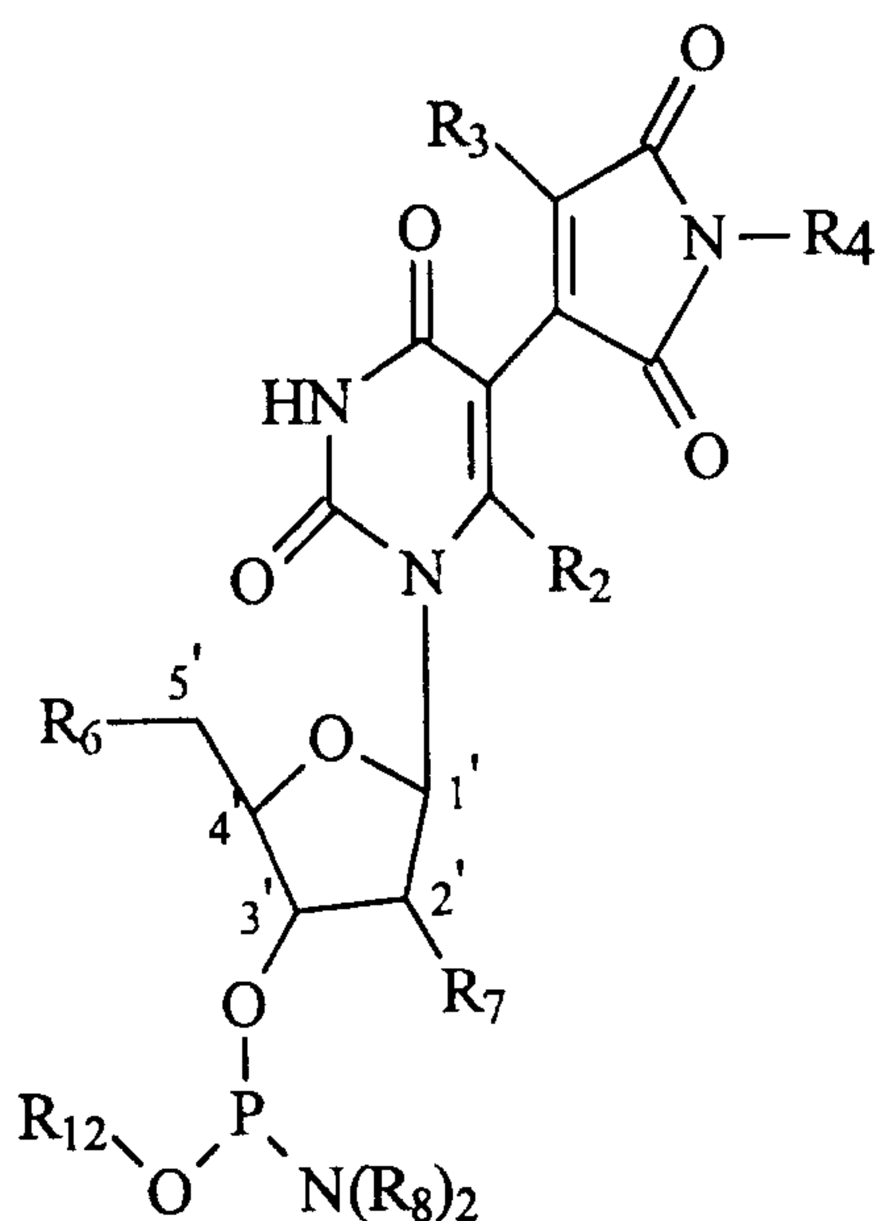
Structure V
