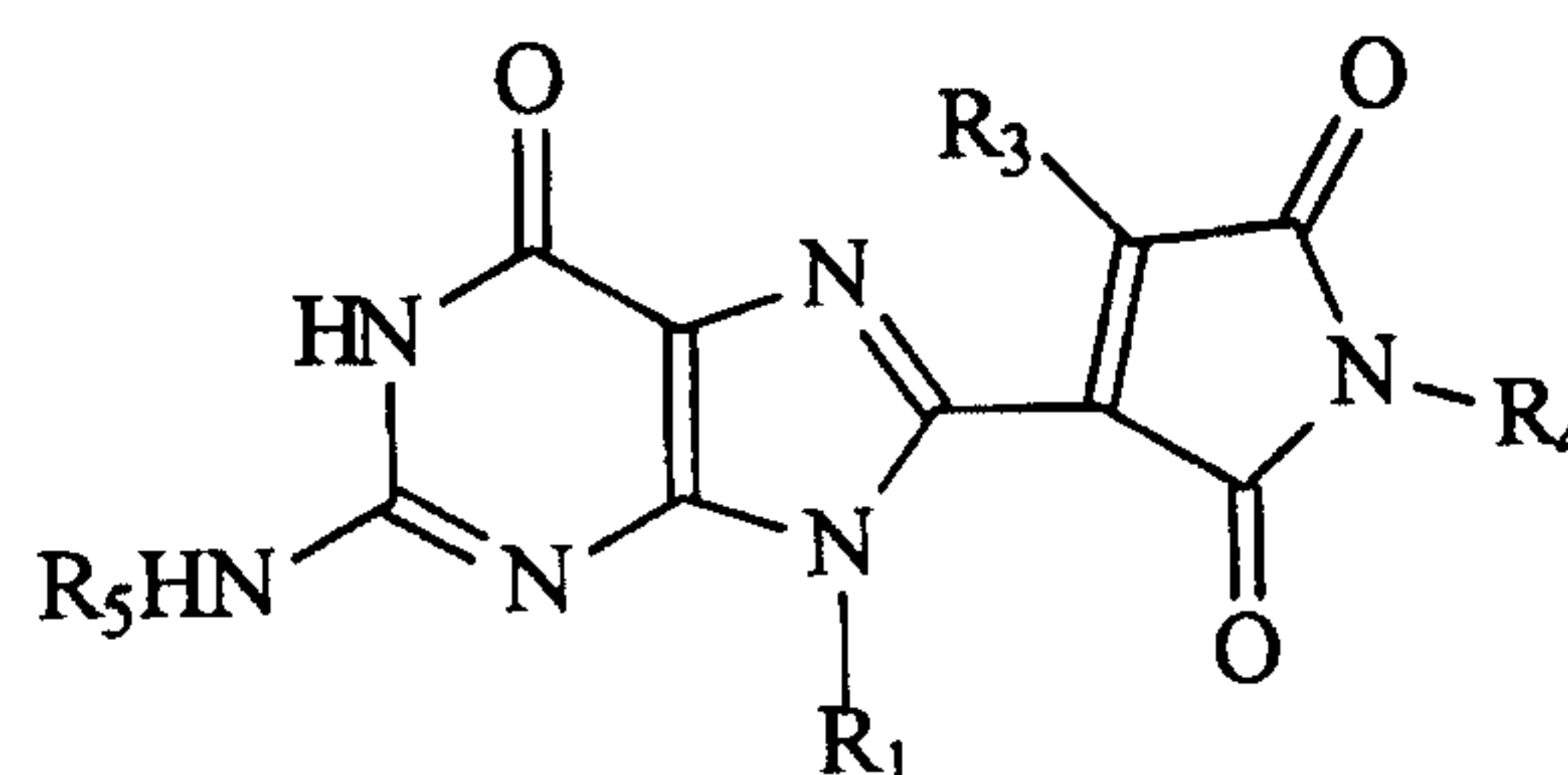
Structure T
