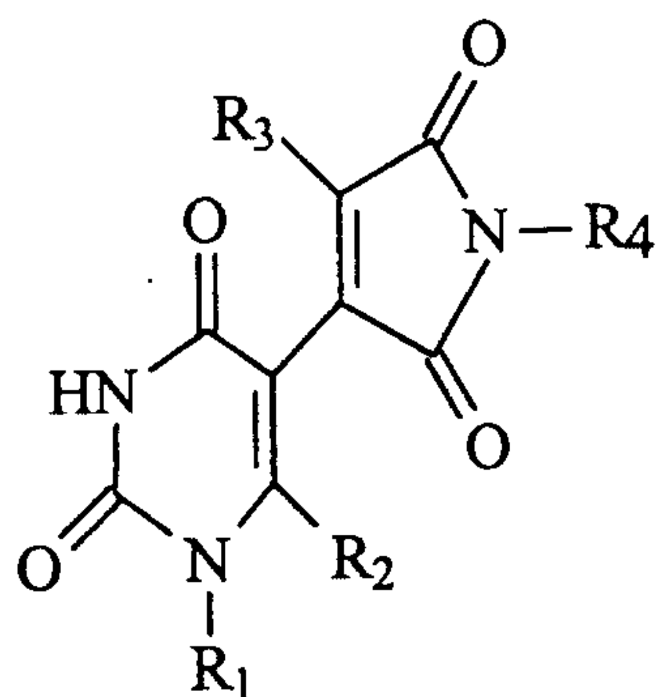
Structure Q
