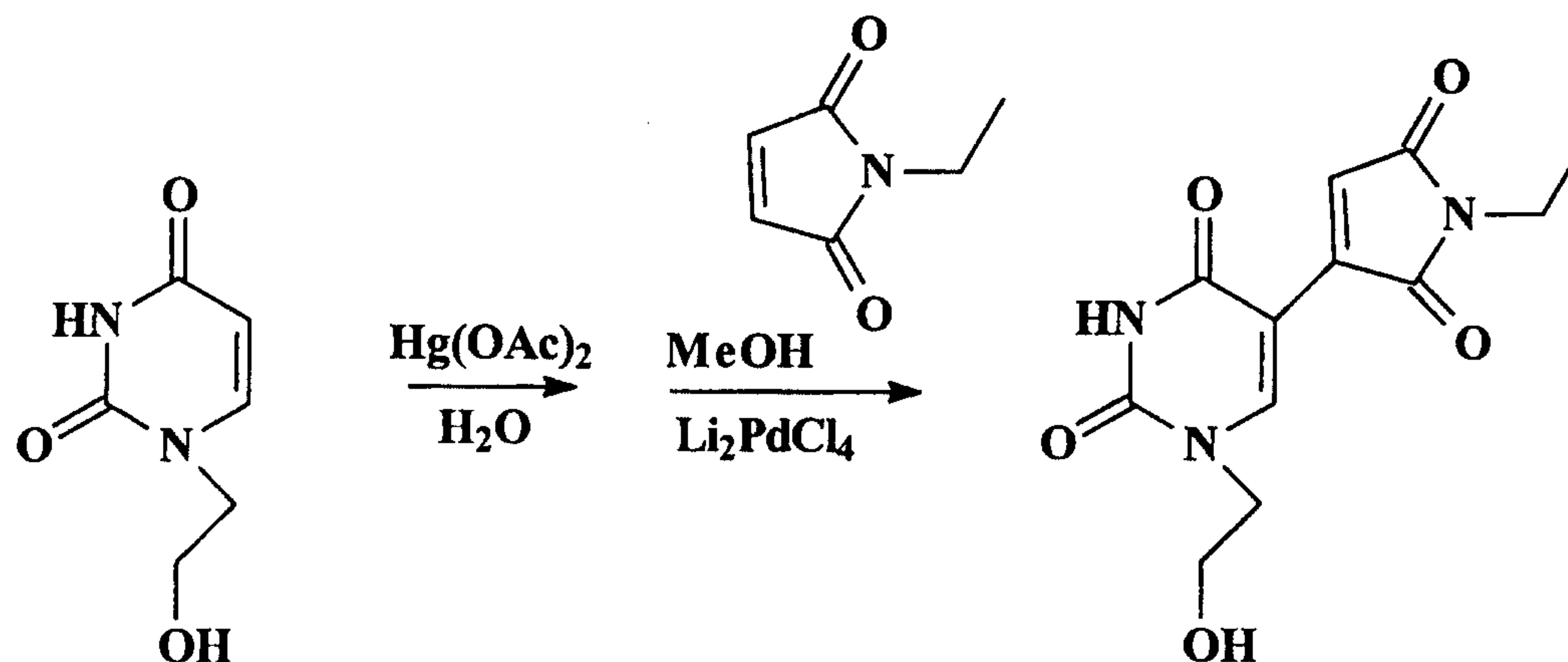
1 - Uracylethanol
