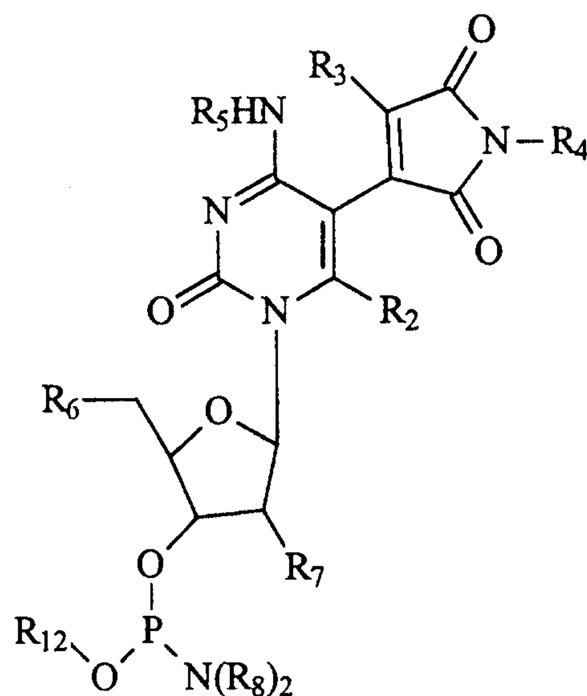
Structure W
