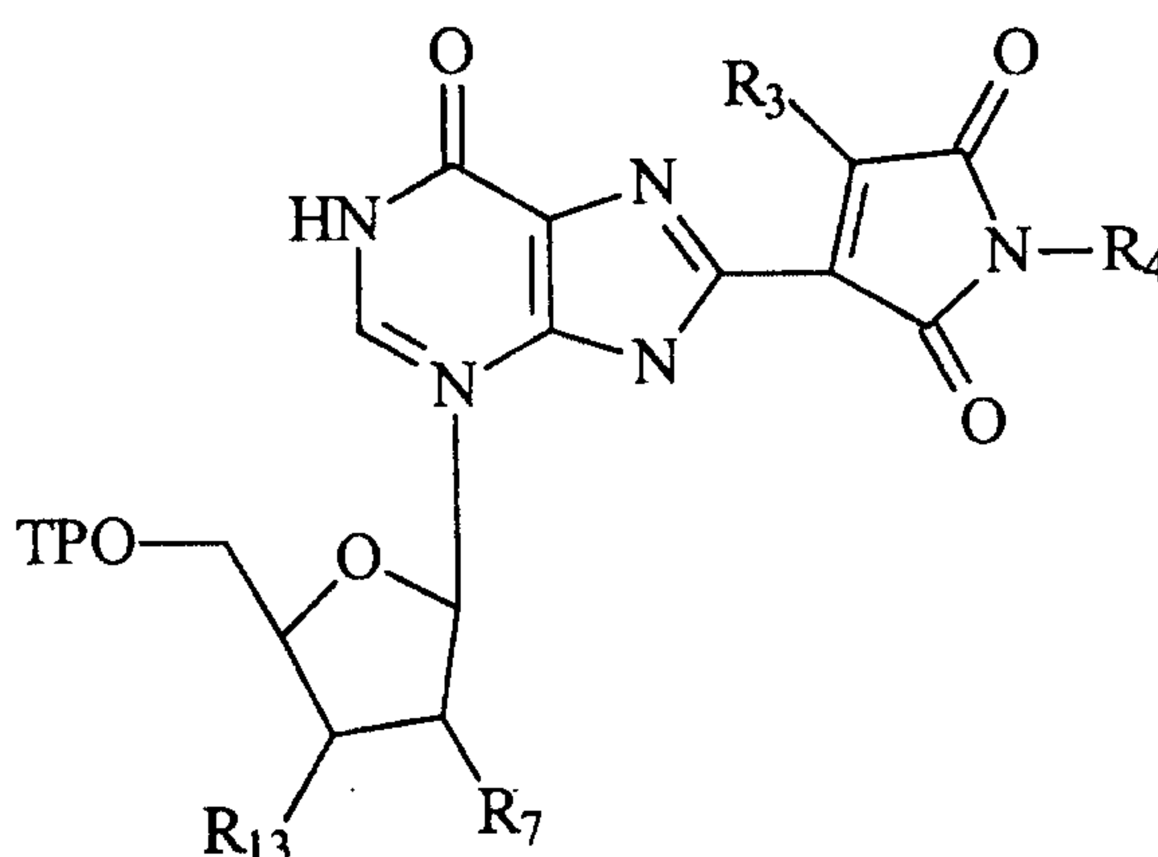
Structure J
