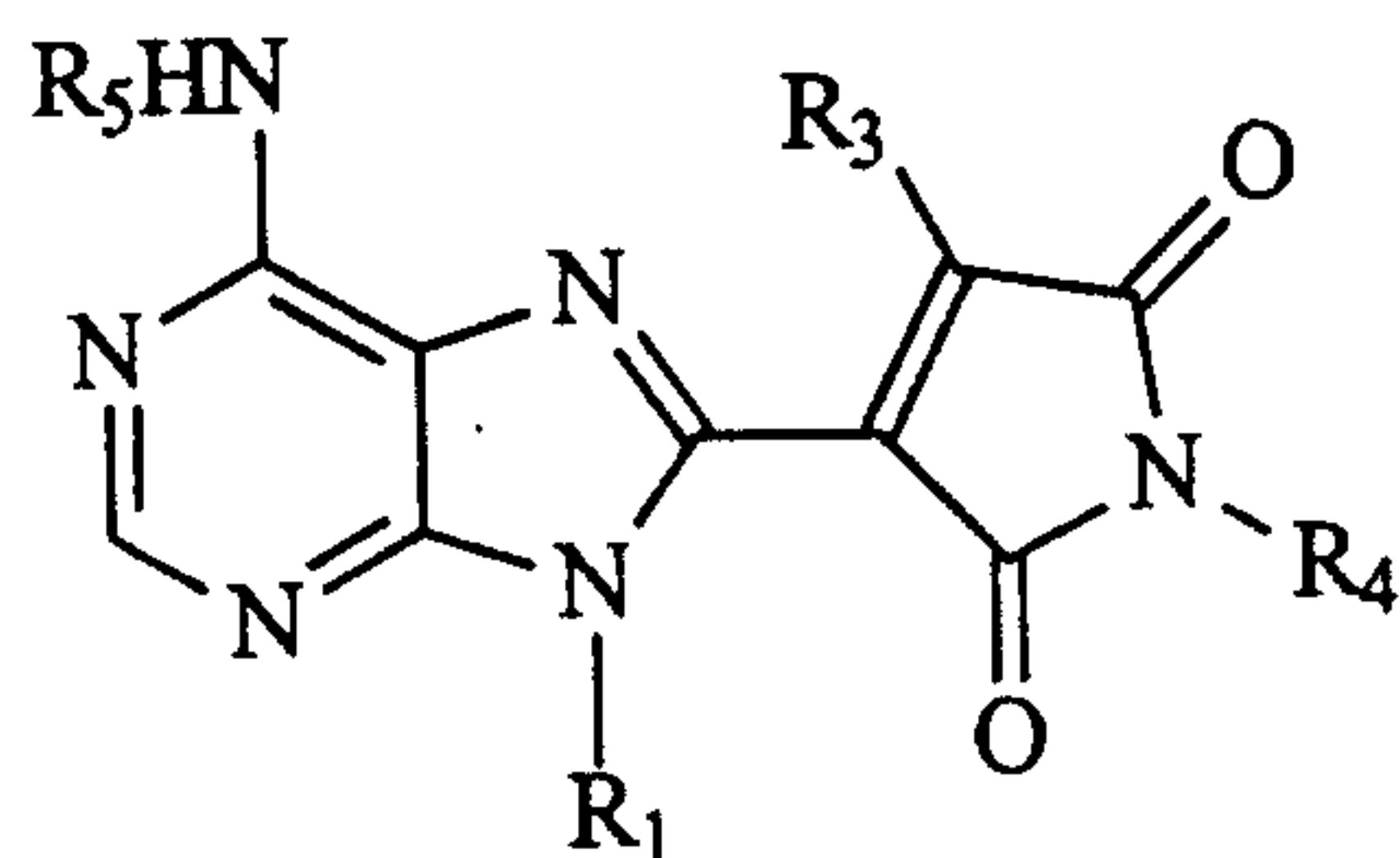
Structure S
