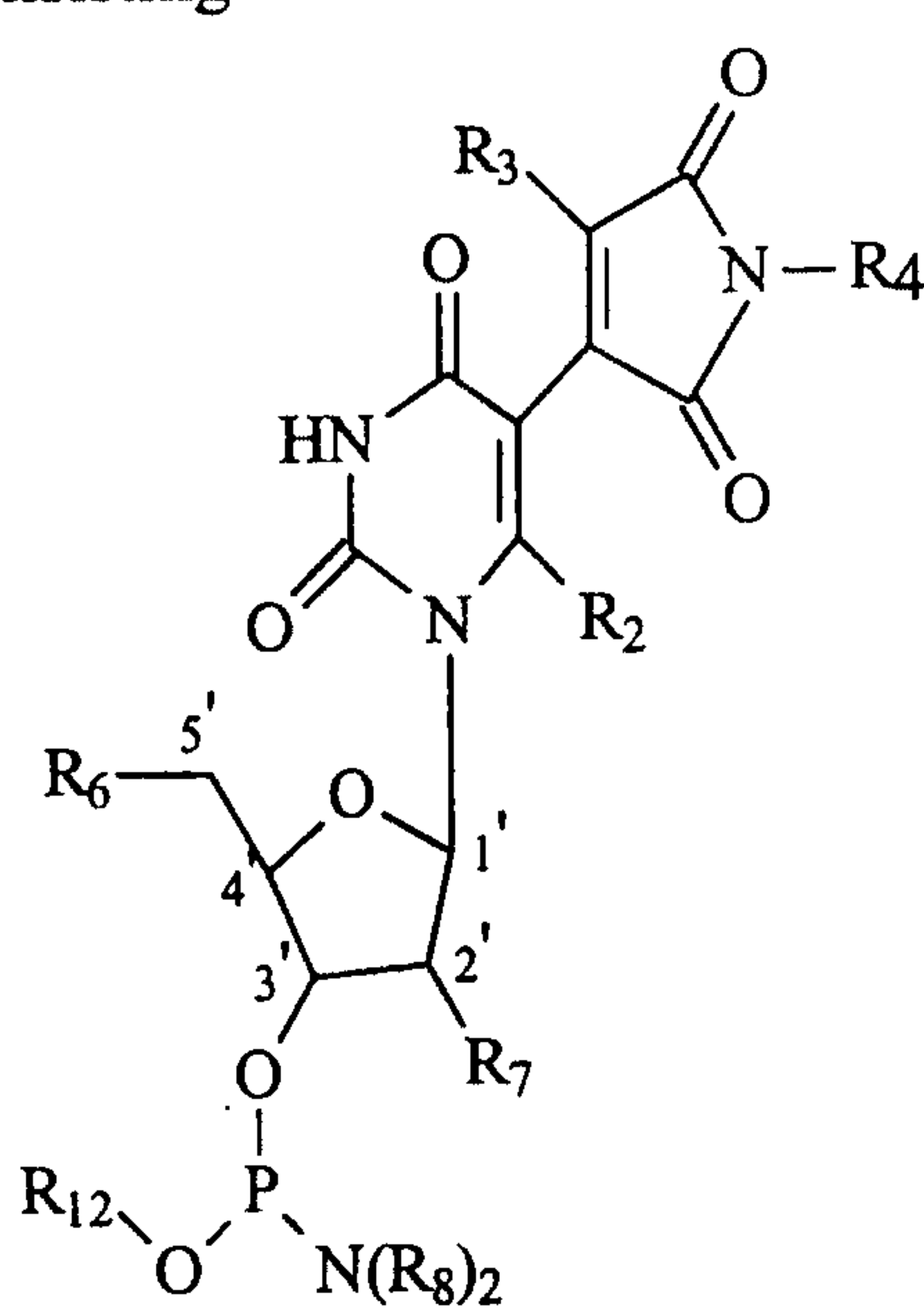
Structure V
