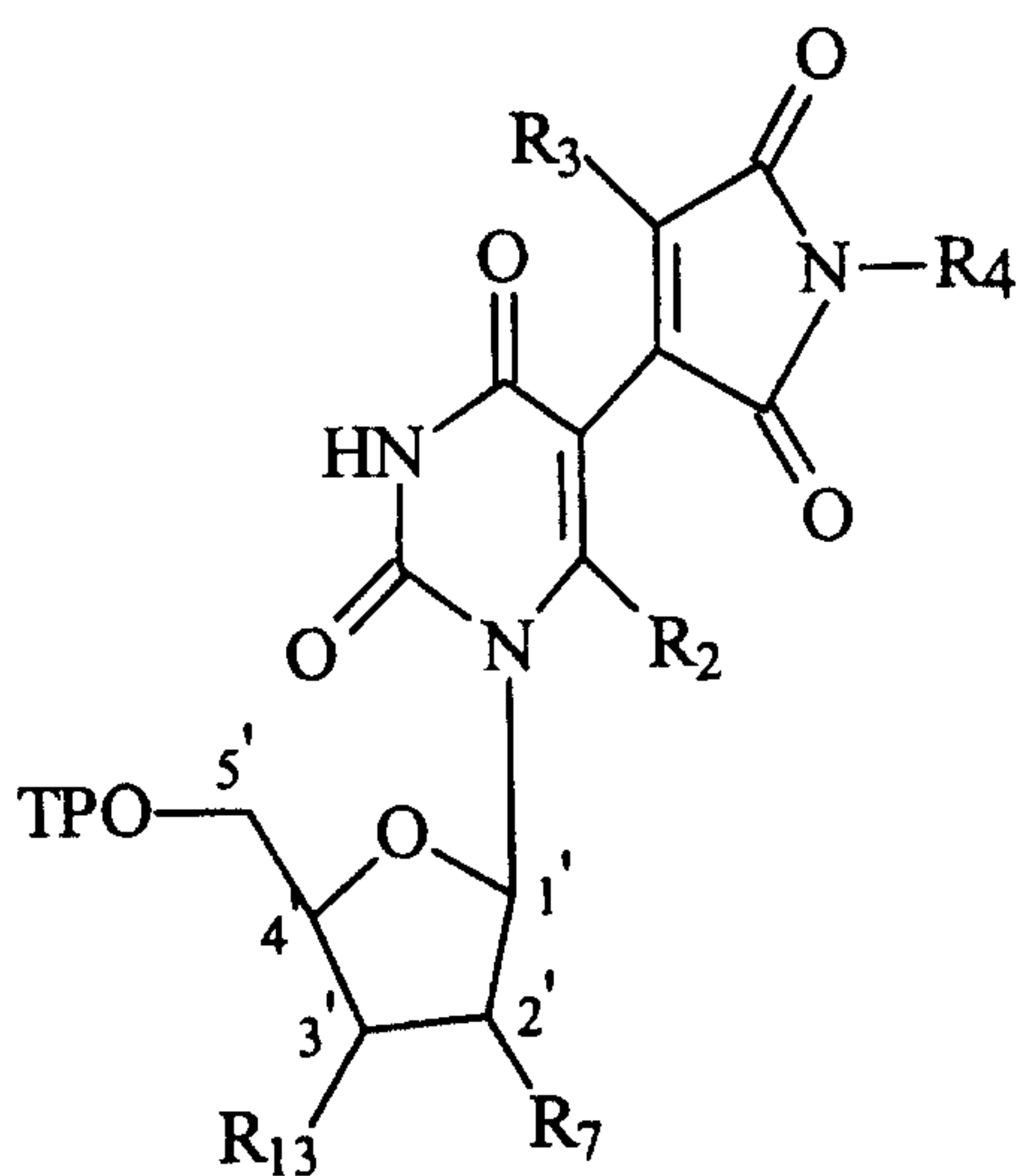
Structure F
