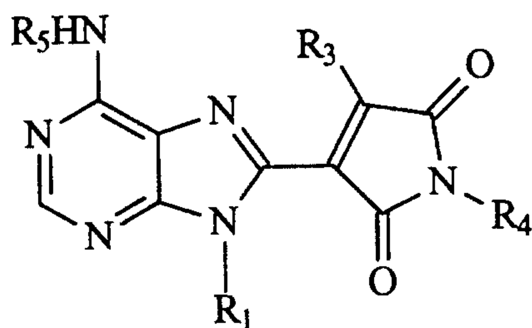
Structure S
