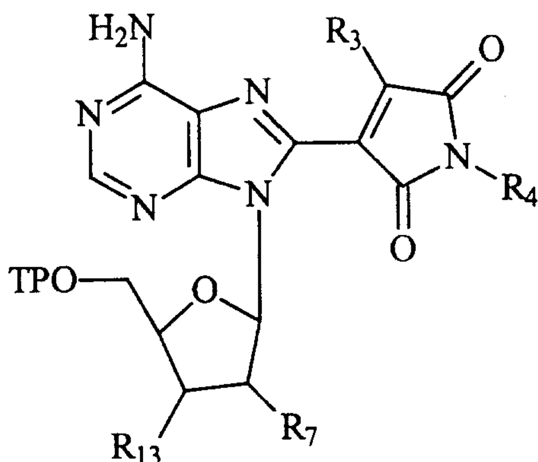
Structure H
