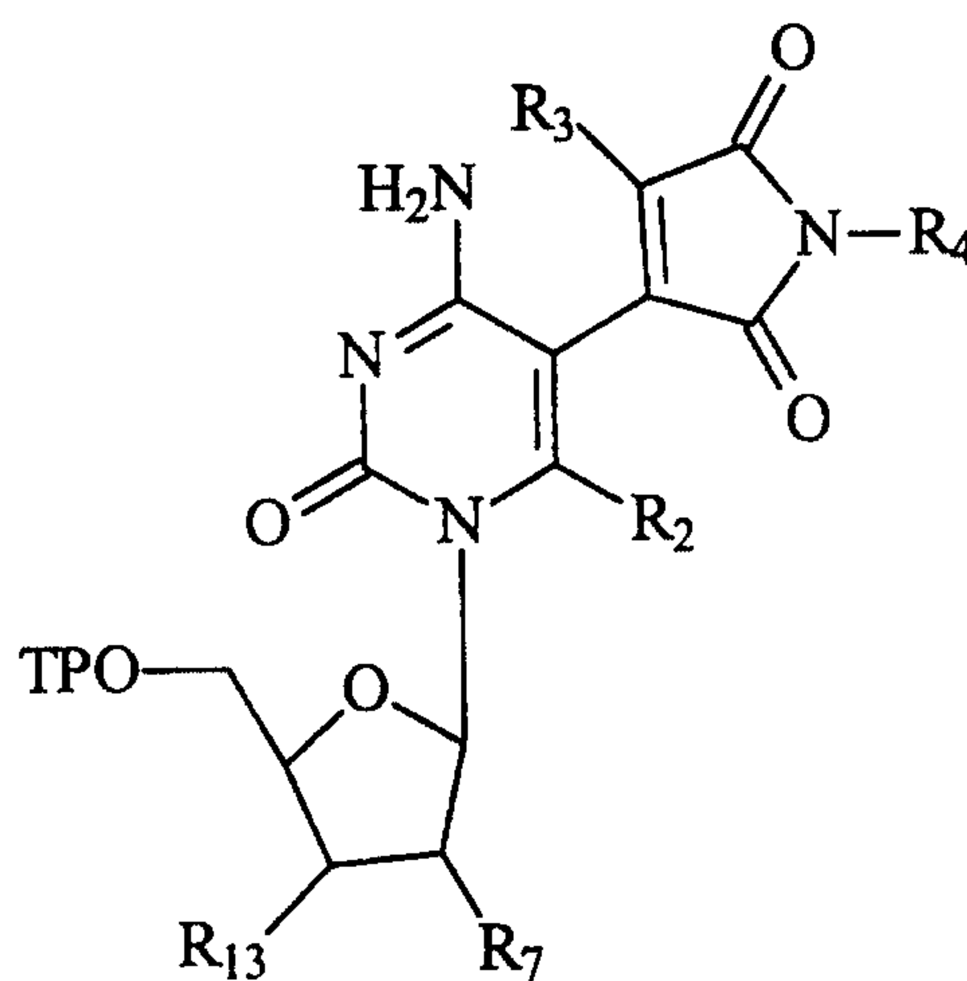
Structure G
