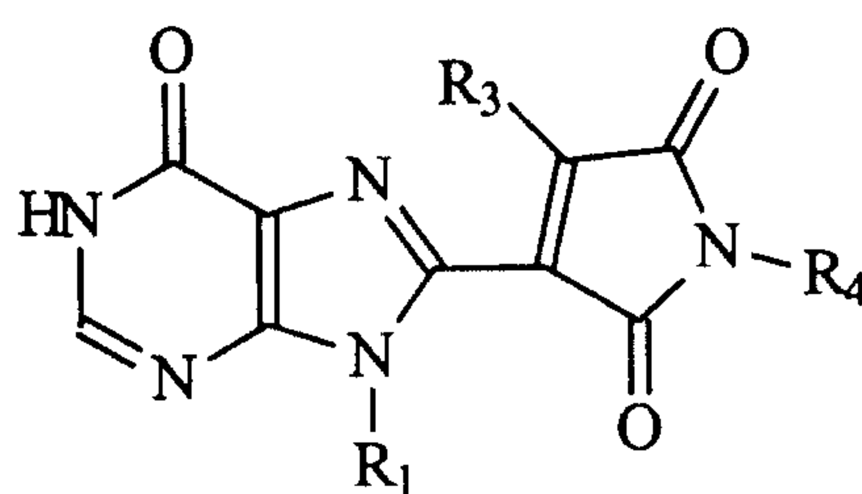
Structure U
