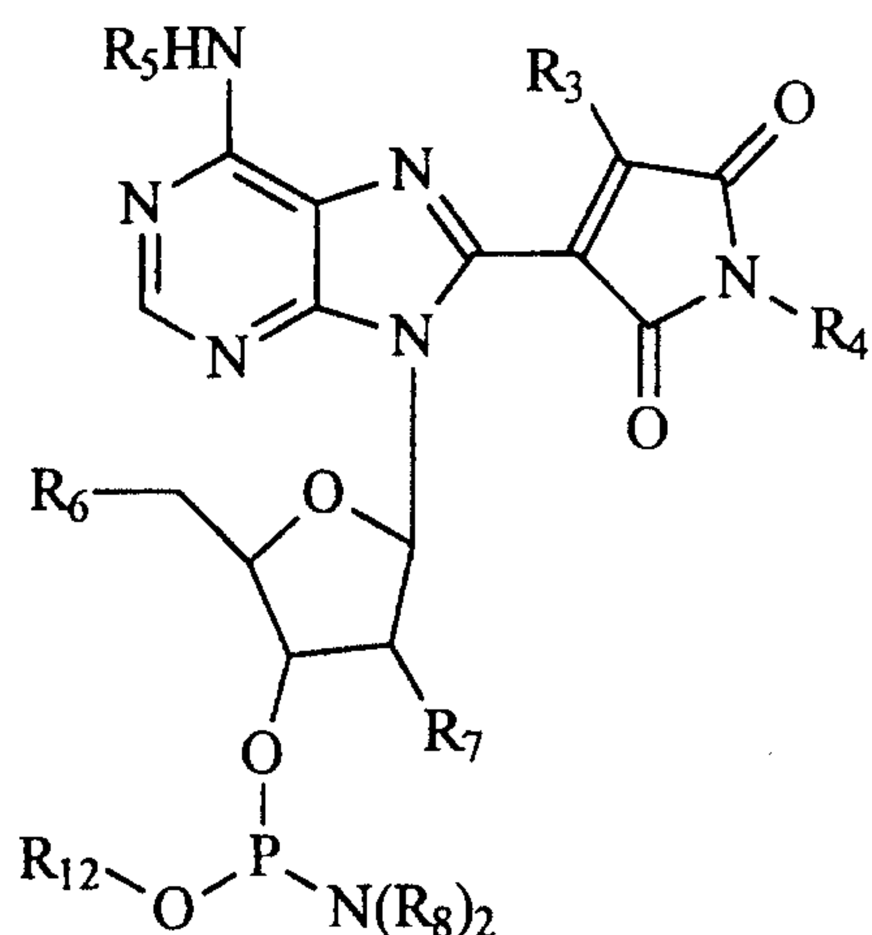
Structure X
