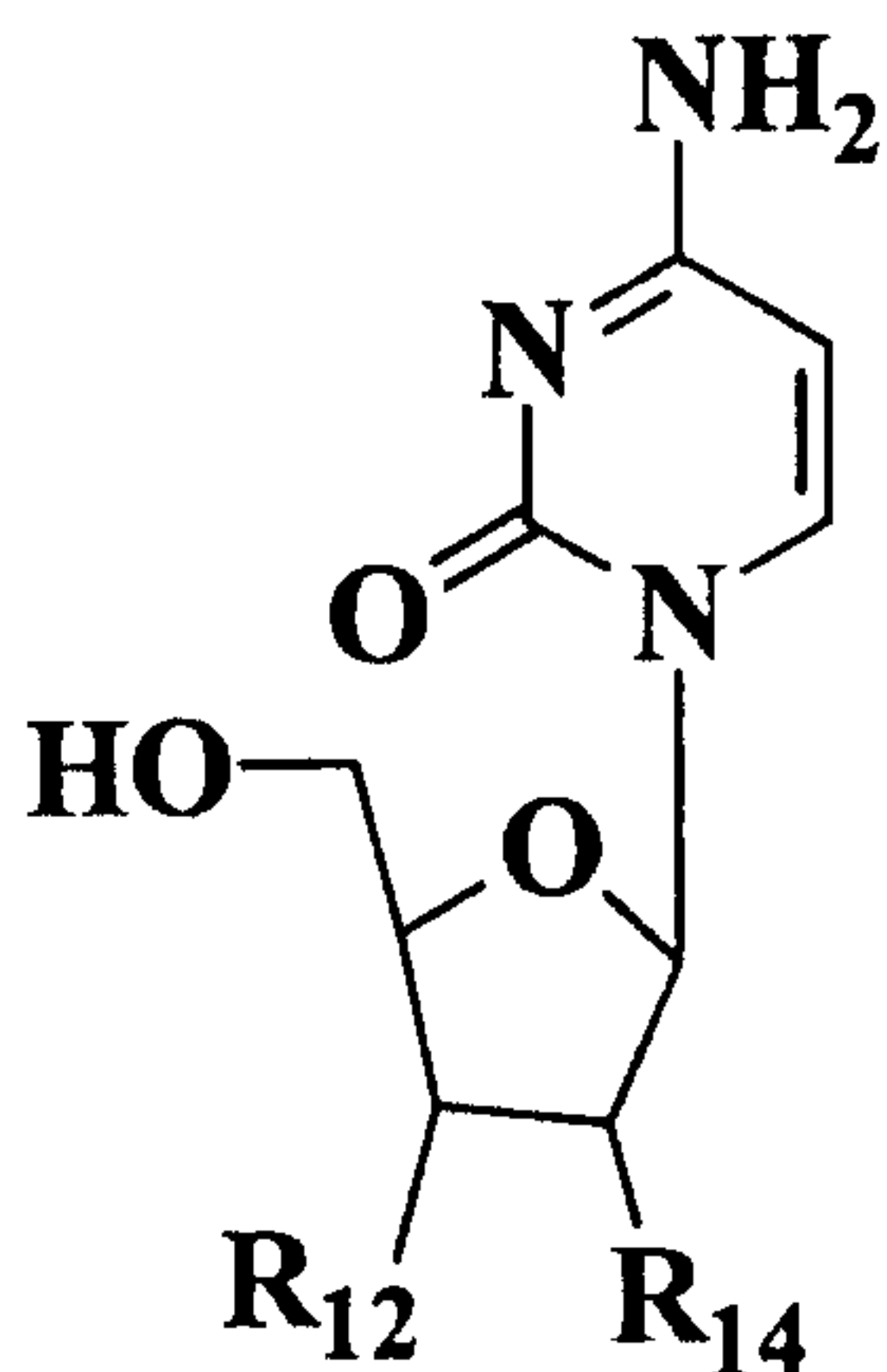
Cytidine
