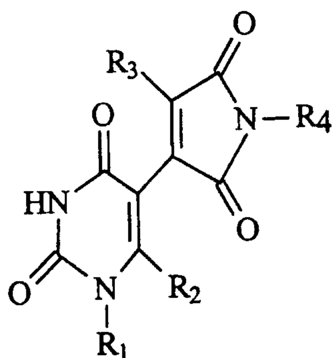
Structure Q
