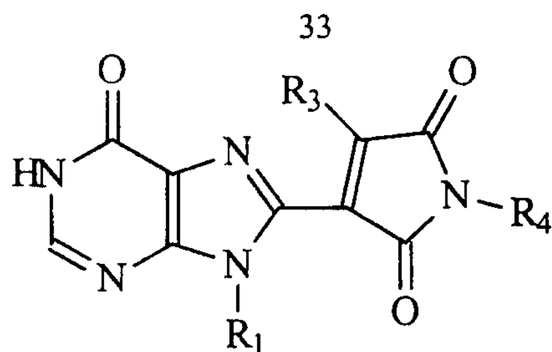
Structure U
