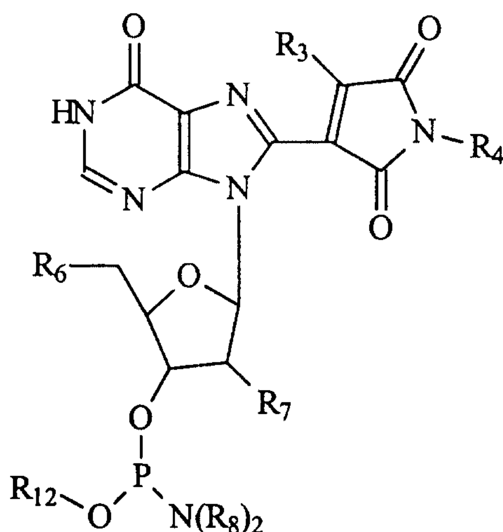
Structure Z
