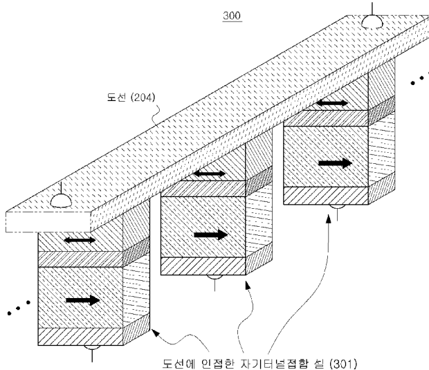
204 ... Wire 301 ... Magnetic tunnel junction cell adjacent to wire
