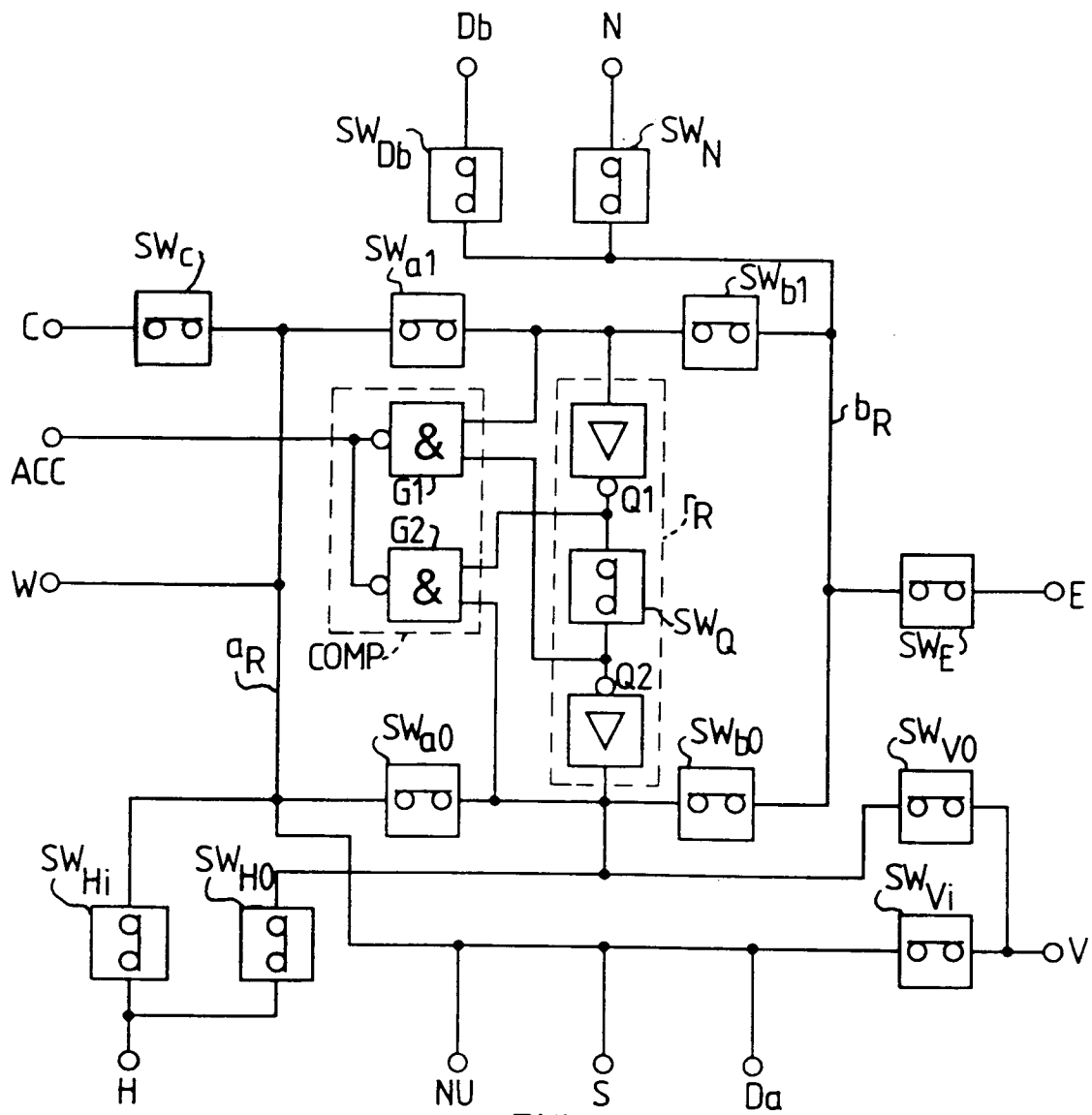
FIG.10 GENERIC REGISTER CELL (NUM & HEAD PLANES)
