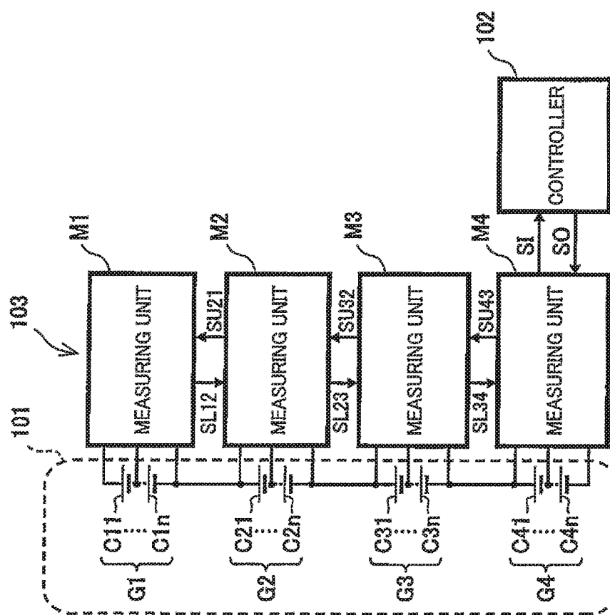
Fig. 5 PRIOR ART
