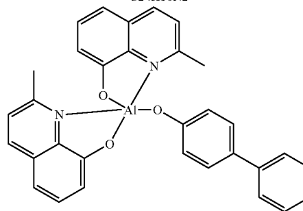
Bis-(2-methyl-8-quinolinolato)-4-(phenyl-phenolato)- aluminium-(III)
