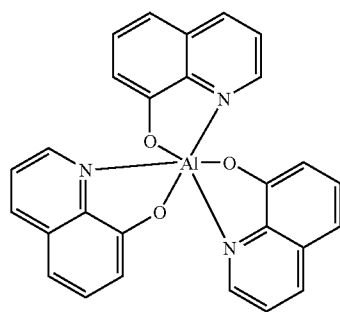
tris (8-hydroxy-quinolinato)-aluminium
