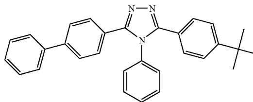
3-(4-Biphenyl)-4-phenyl-5-tert- butylphenyl-1,2,4-triazole C 30 H 27 N 3
