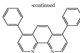
BPhen = bathophenanthroline (4,7-Diphenyl-1,10-phenanthroline) C 24 H 16 N 2
