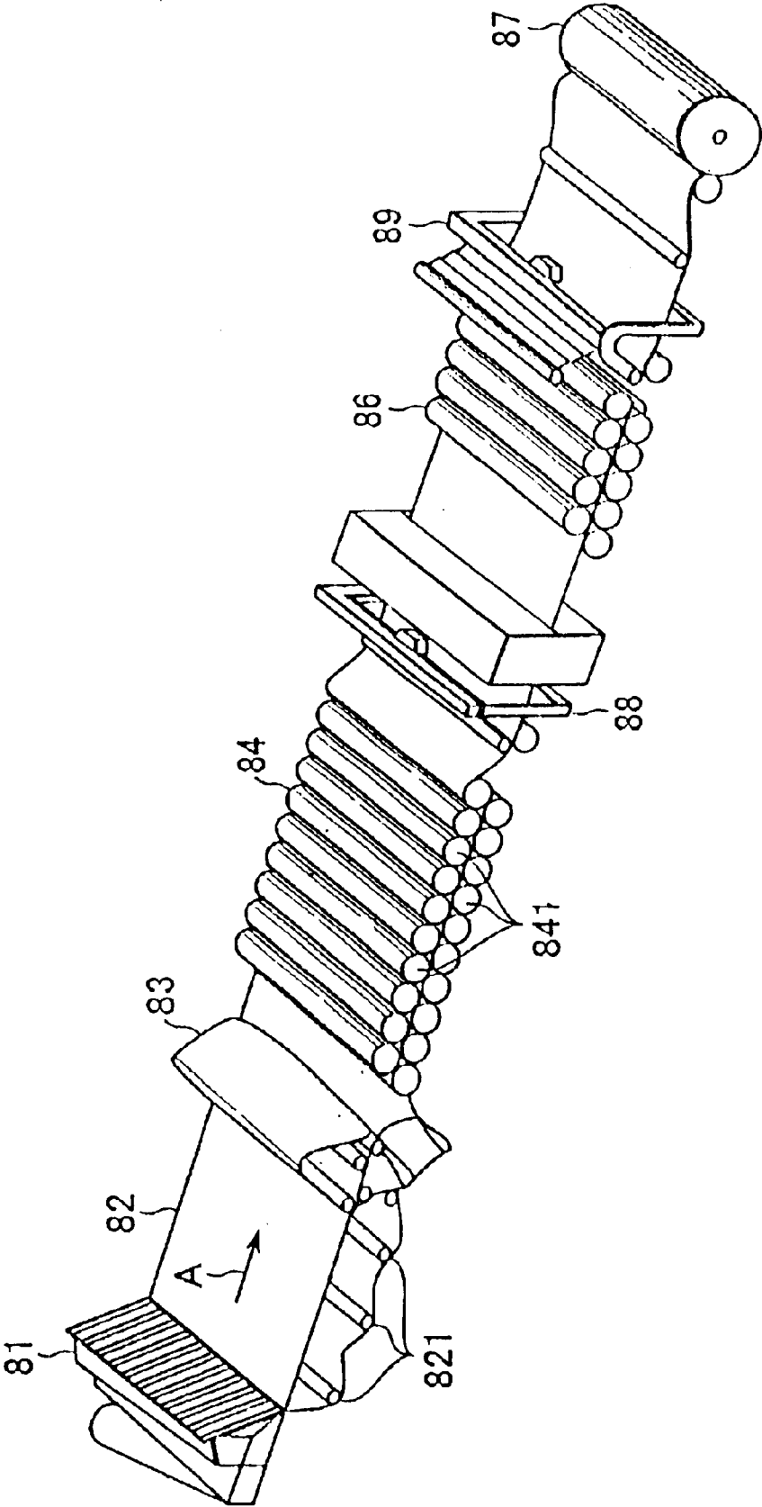
FIG. 1 (PRIOR ART)
