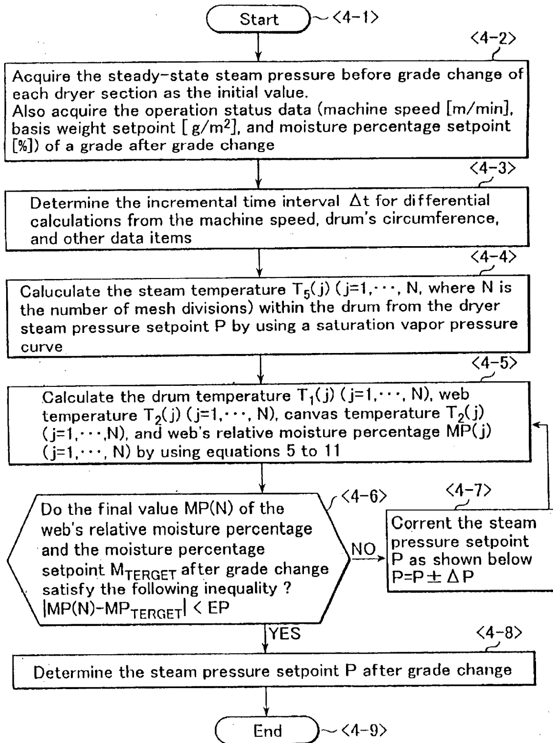
FIG. 4 (PRIOR ART)
