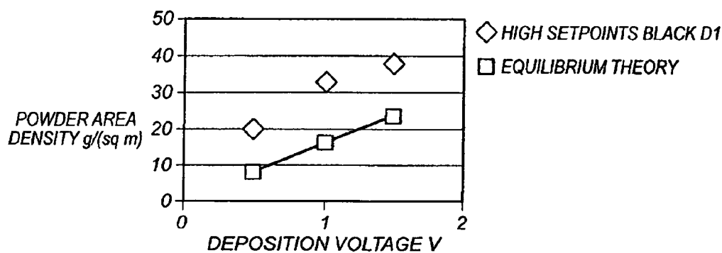
POWDER AREA DENSITY VS. DEPOSITION VOLTAGE
