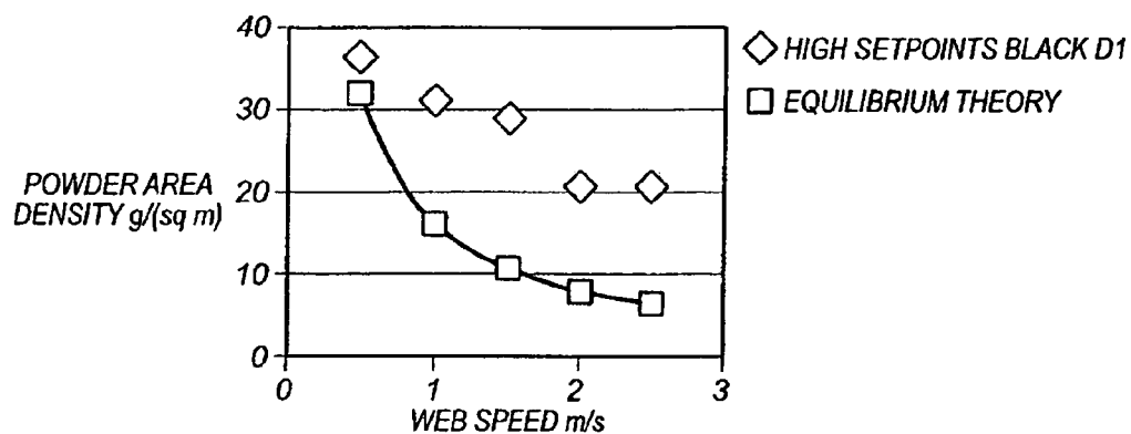
POWDER AREA DENSITY VS. WEB SPEED
