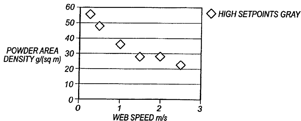
POWDER AREA DENSITY VS. WEB SPEED
