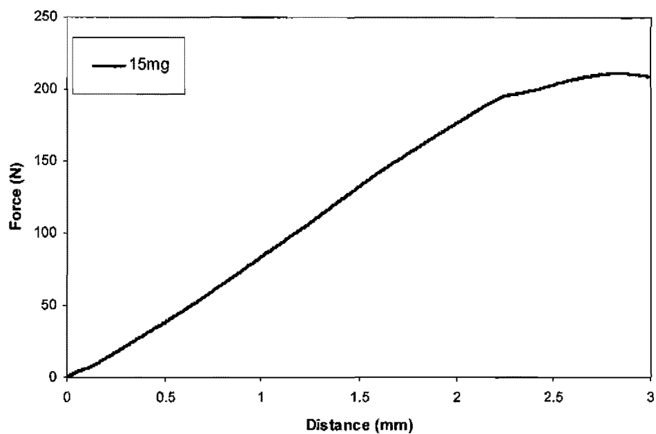
Example 20 Indentation Test of Example 14.2 tablet
