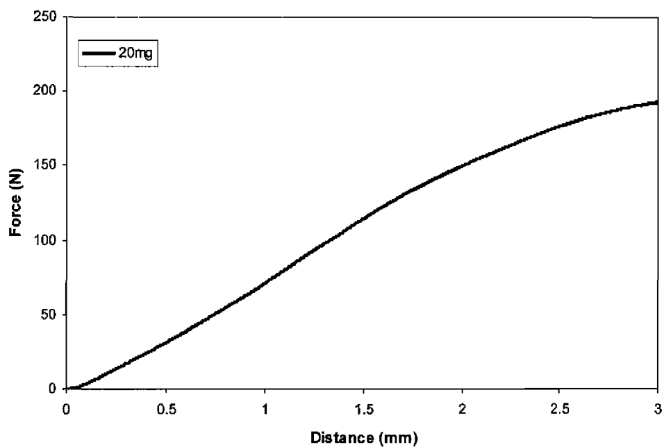
Example 20 Indentation Test of Example 13.3 tablet
