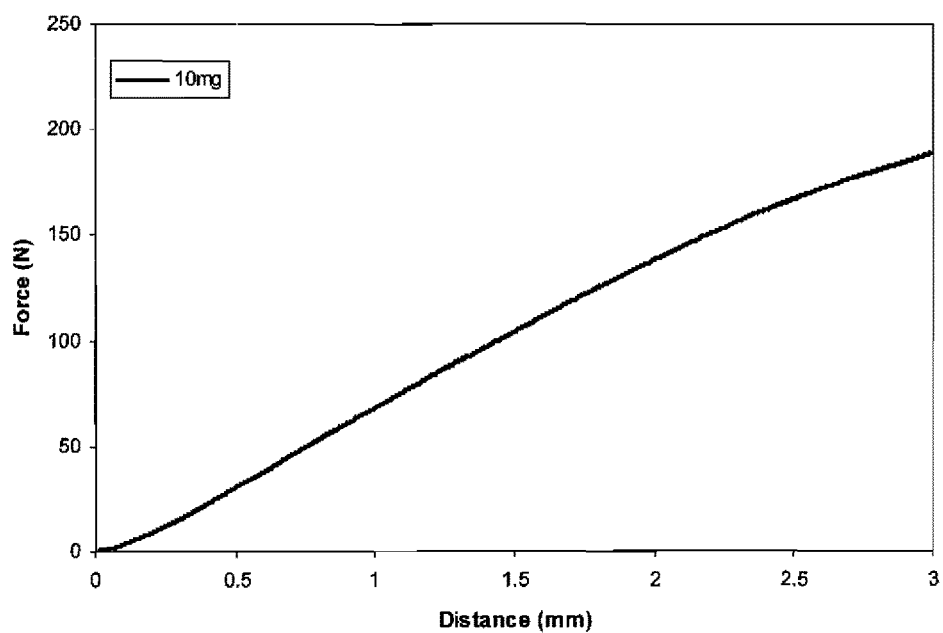
Example 20 Indentation Test of Example 13.1 tablet
