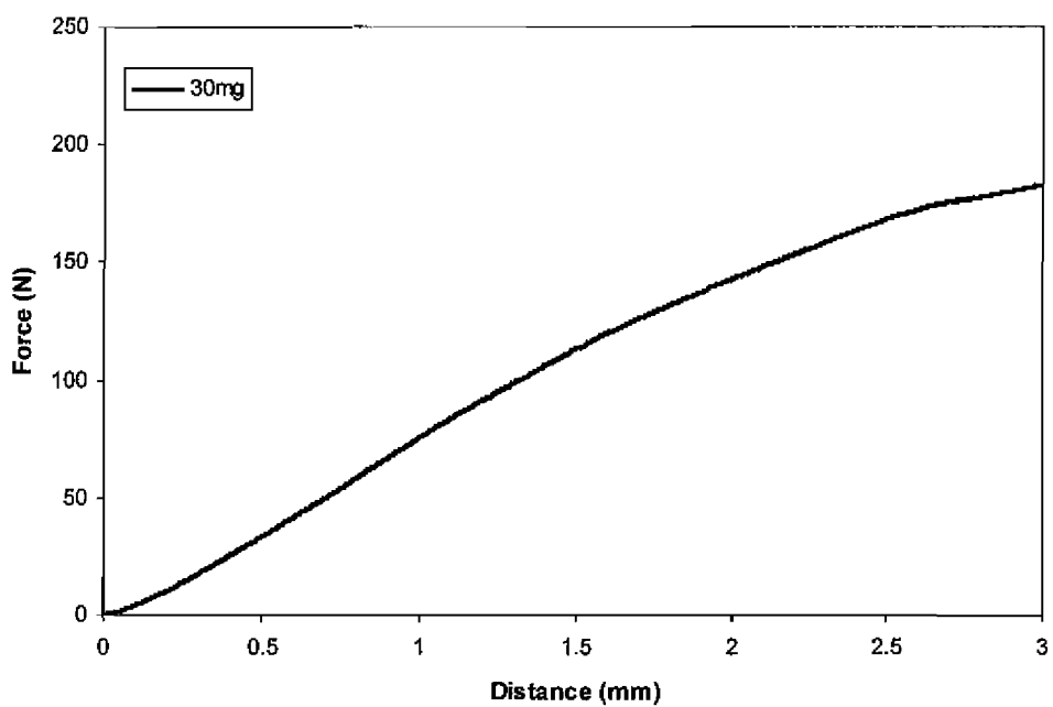
Example 20 Indentation Test of Example 13.4 tablet
