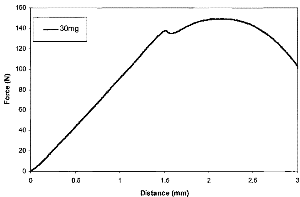
Example 20 Indentation Test of Example 14.4 tablet
