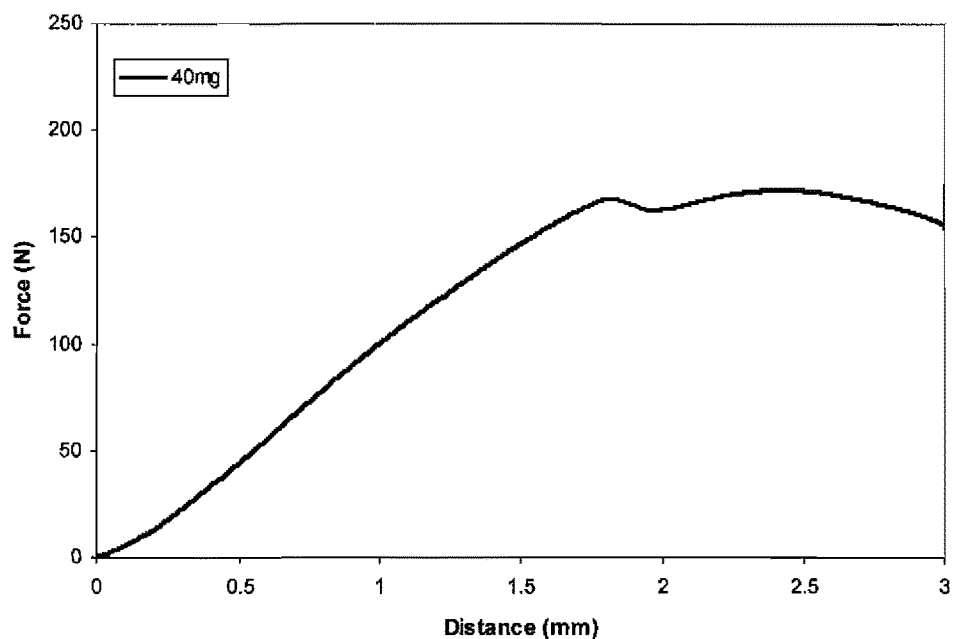
Example 20 Indentation Test of Example 13.5 tablet
