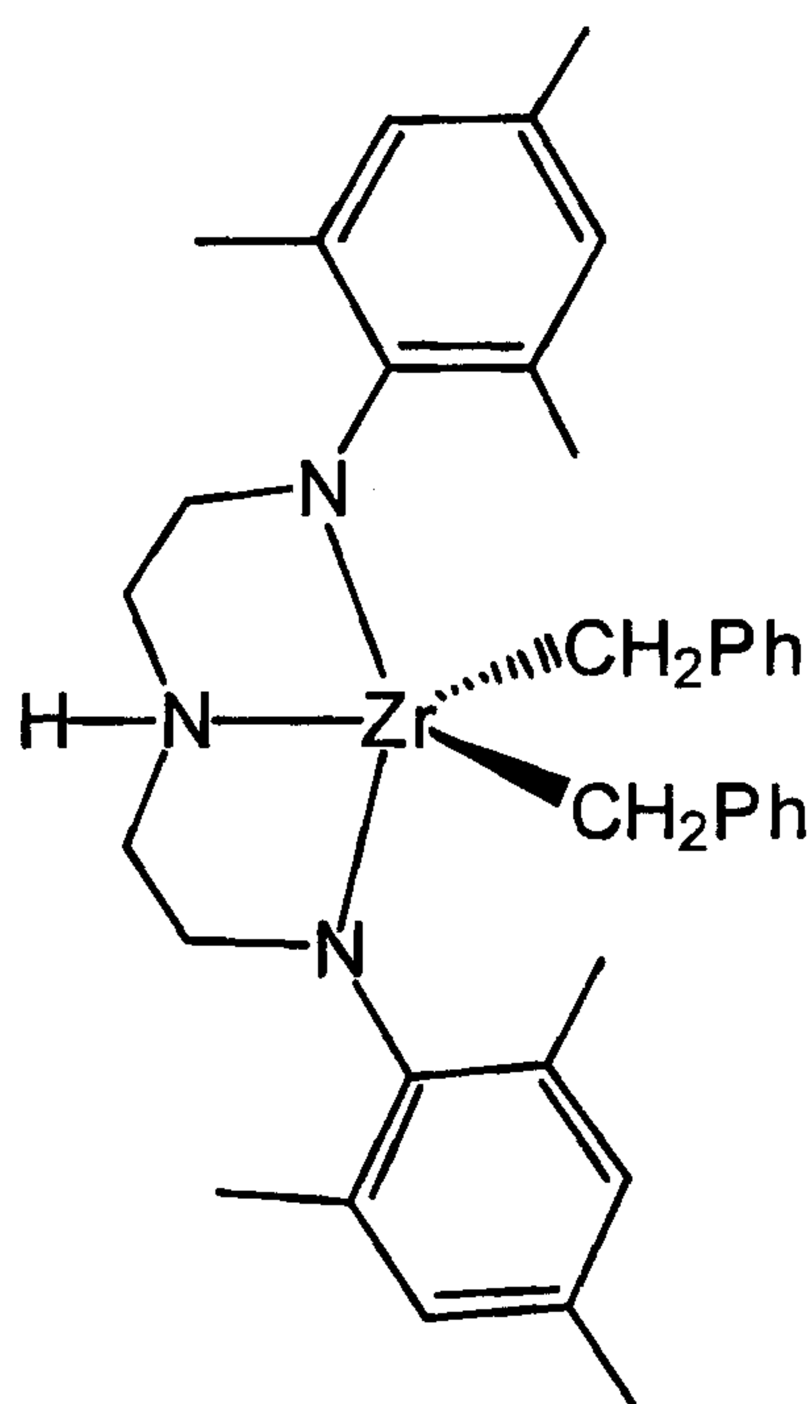
Compound I
