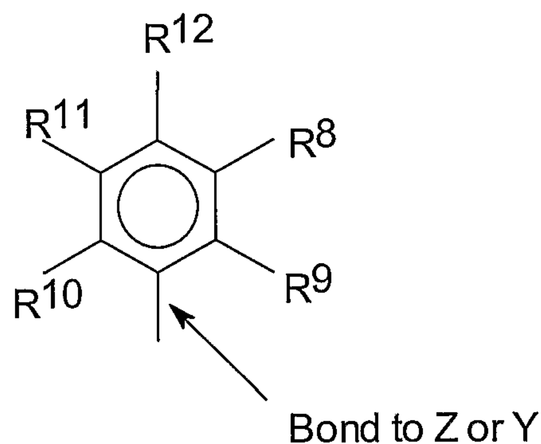
Formula 1
