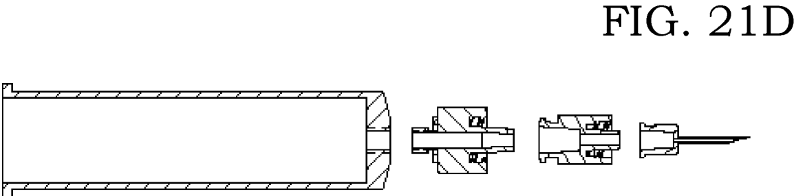
Exploded View
