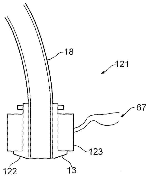
Vibrating nozzle
