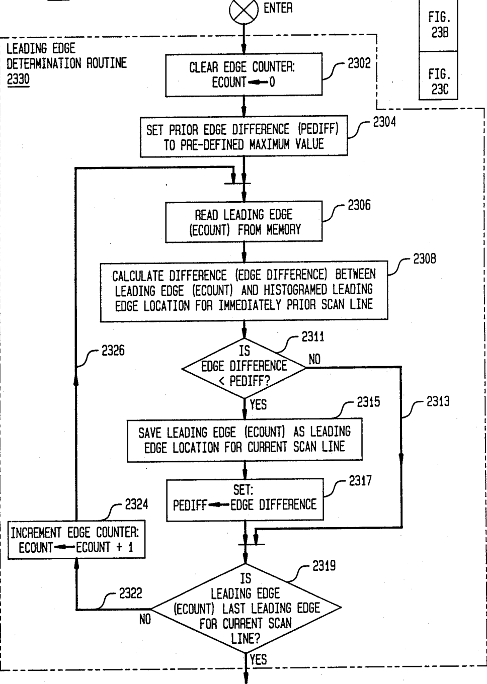
FIG. 23A PRIOR LINE EDGE PAIR SELECTION ROUTINE 2300
