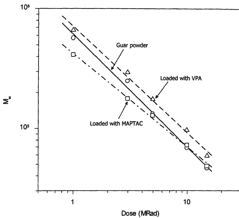
Depolymerization of Guar.
