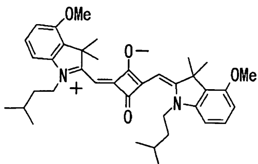
Compound No.9
