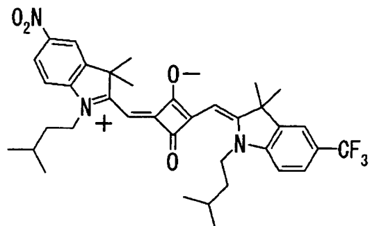
Compound No.12
