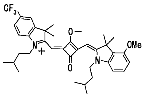
Compound No.14
