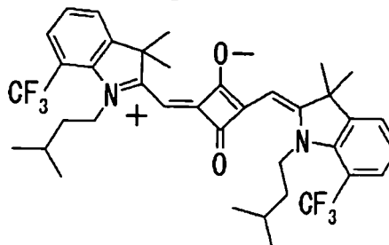
Compound No.20
