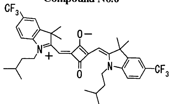
Compound No.6
