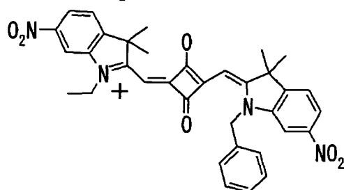
Compound No.36
