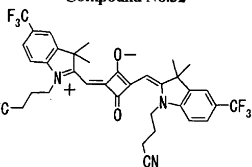
Compound No.34
