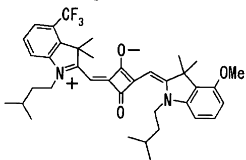
Compound No.13
