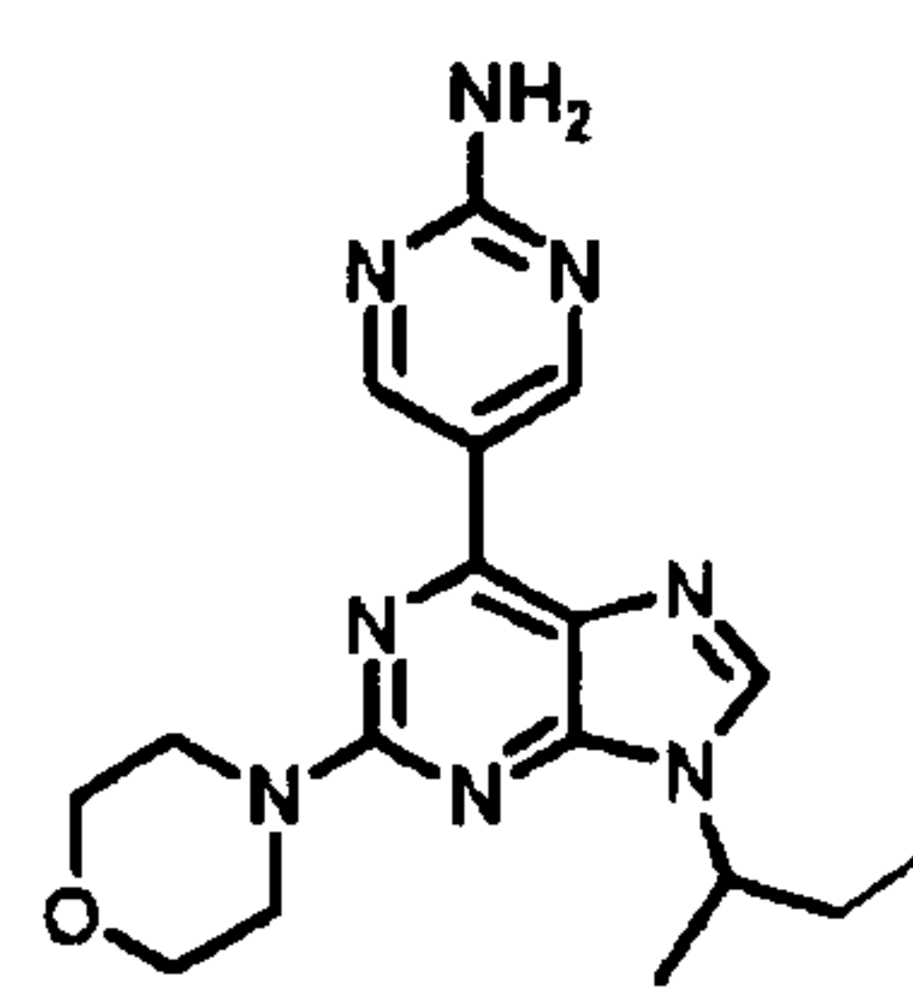
Compound E
