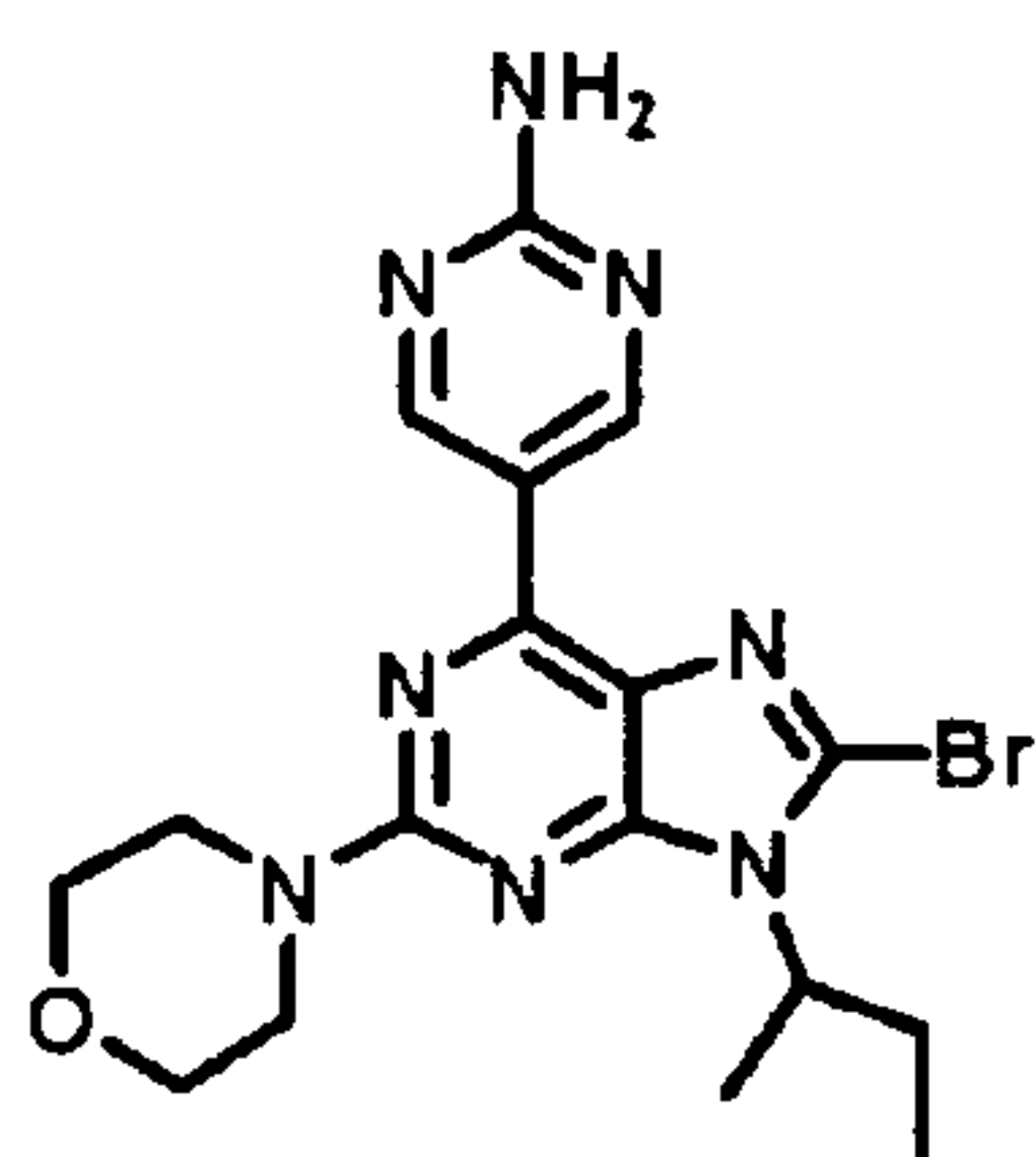
Compound A
