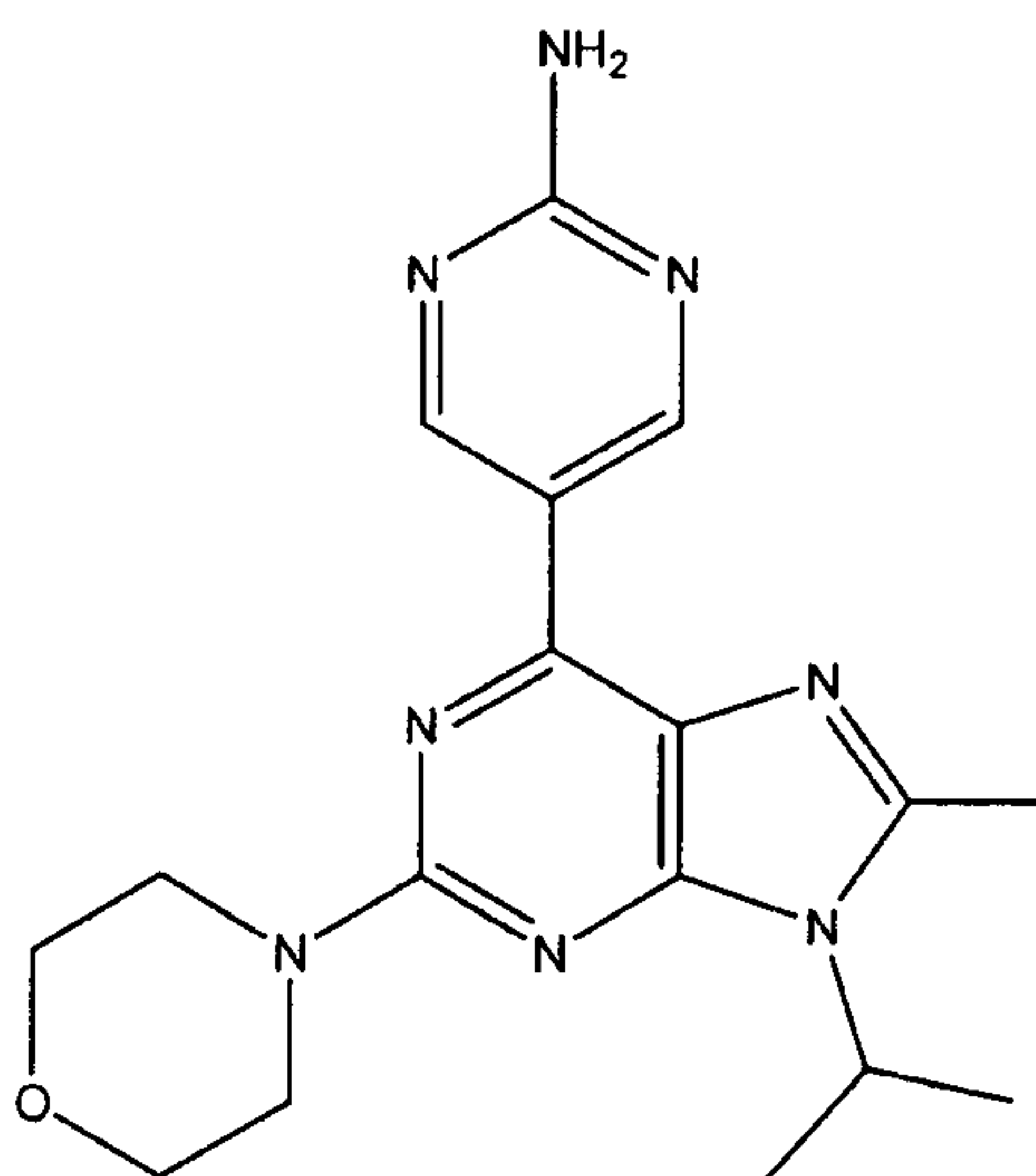
Formula (I)
