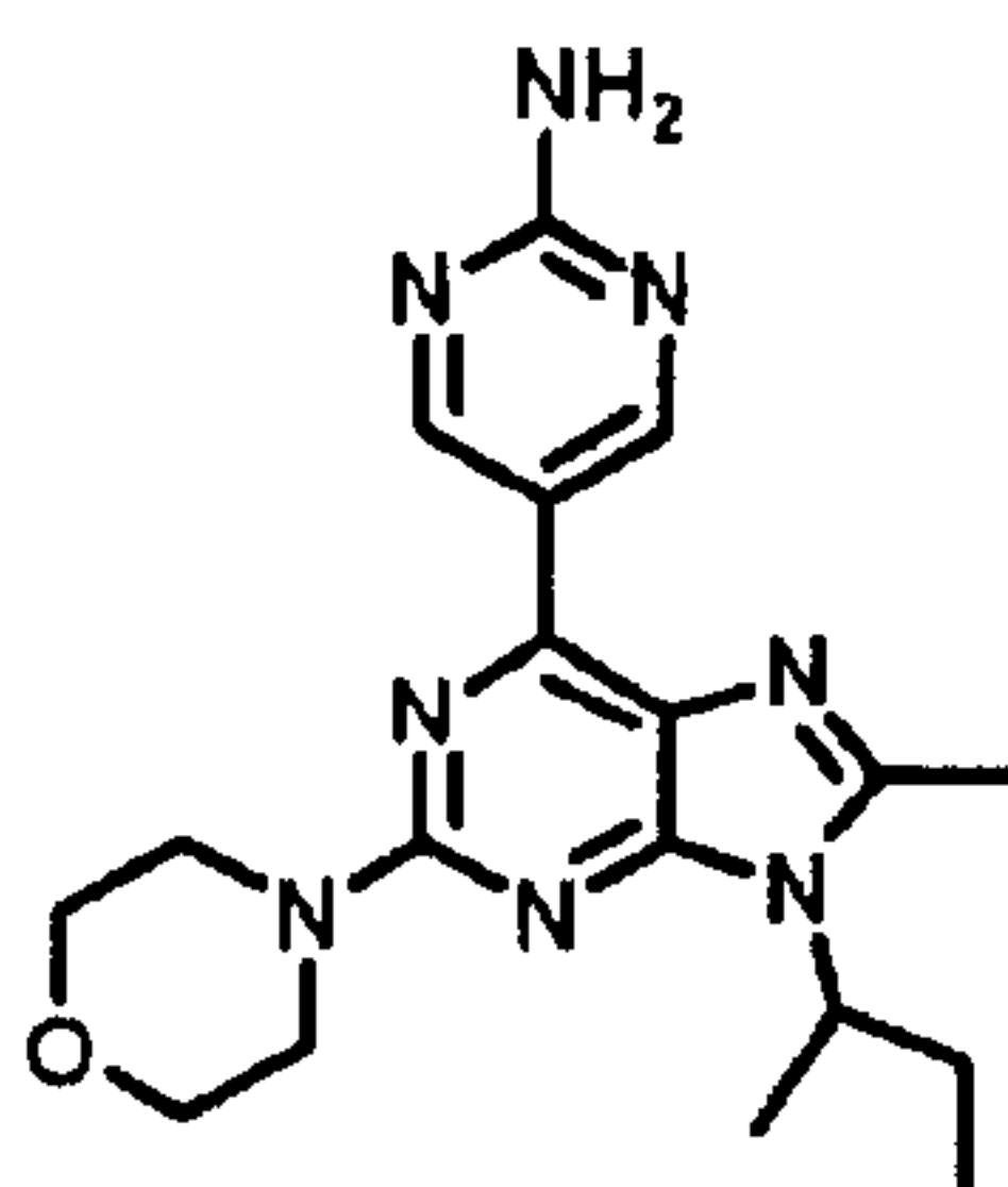
Compound D
