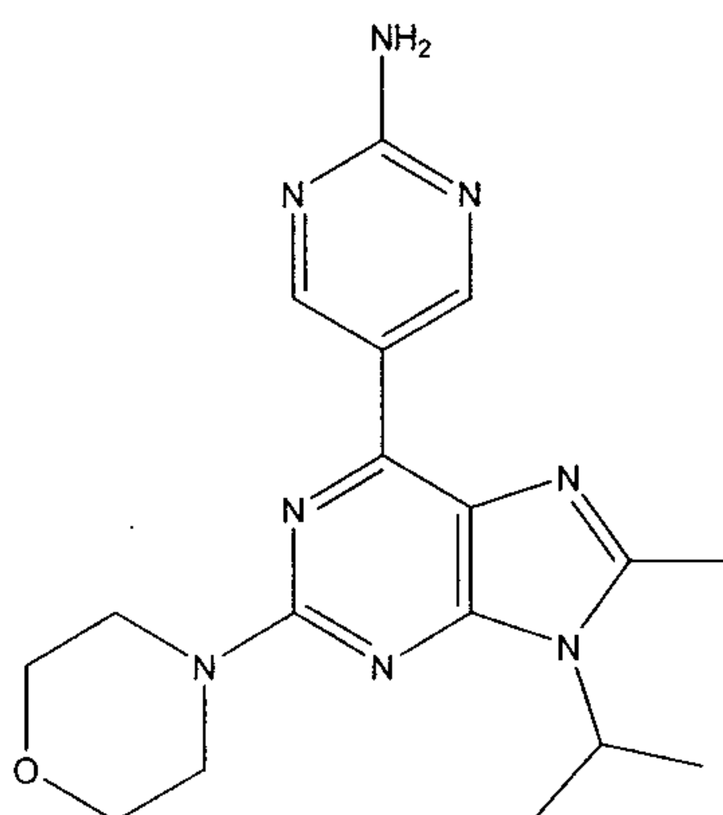
Formula (I)
