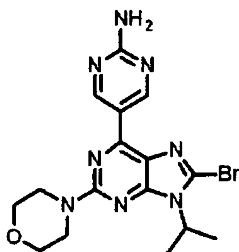
Compound B
