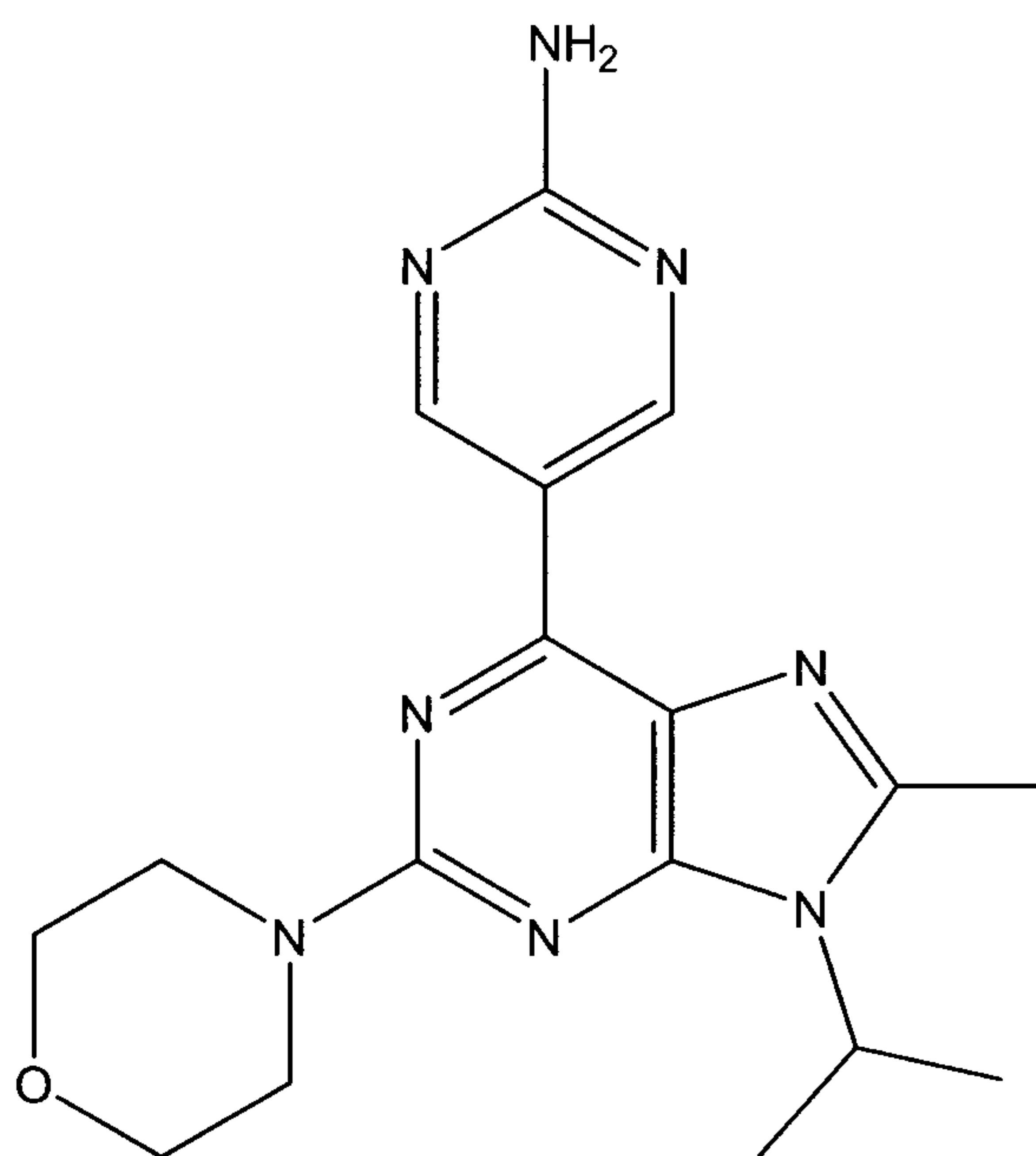
Formula (I)
