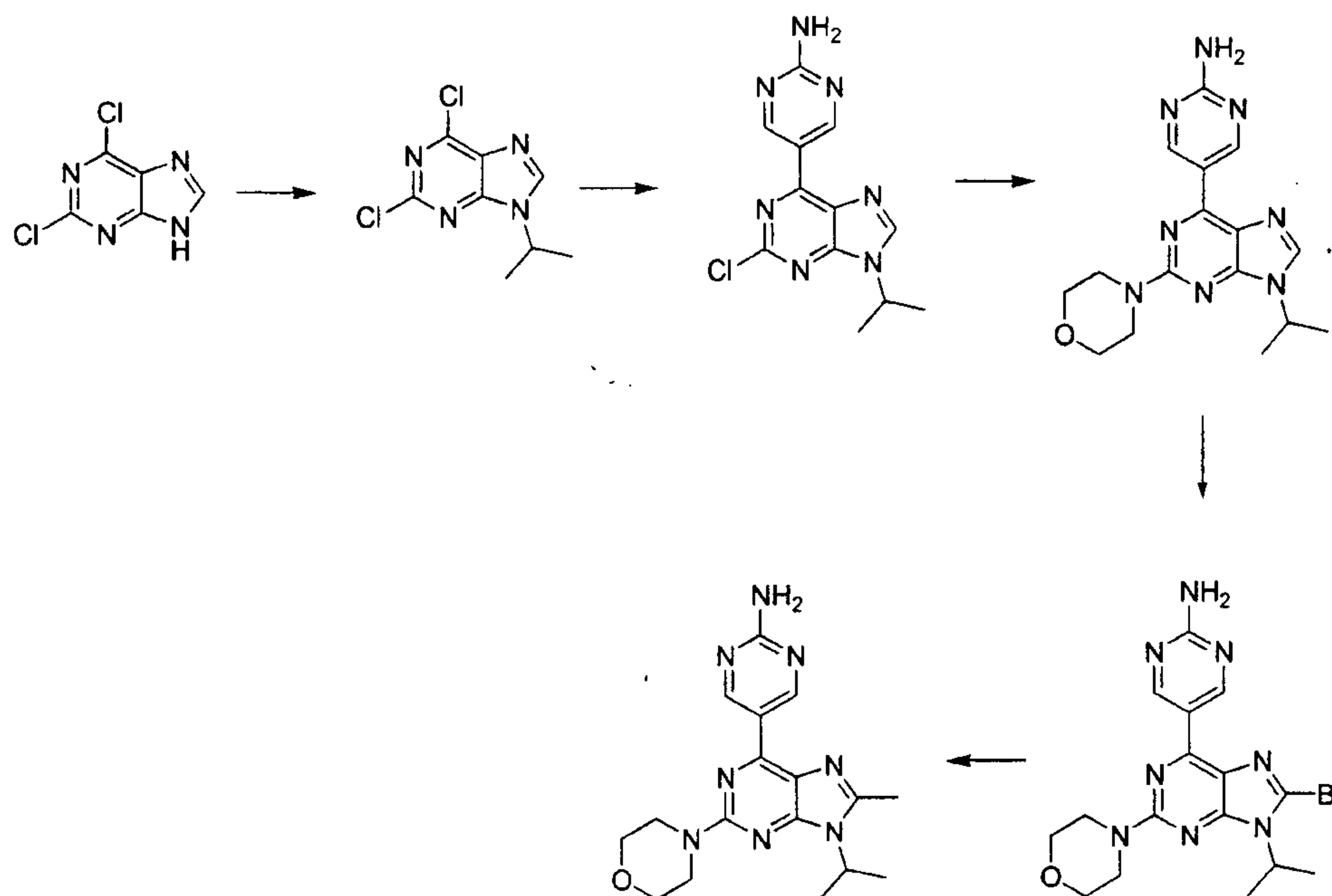
Scheme 1
