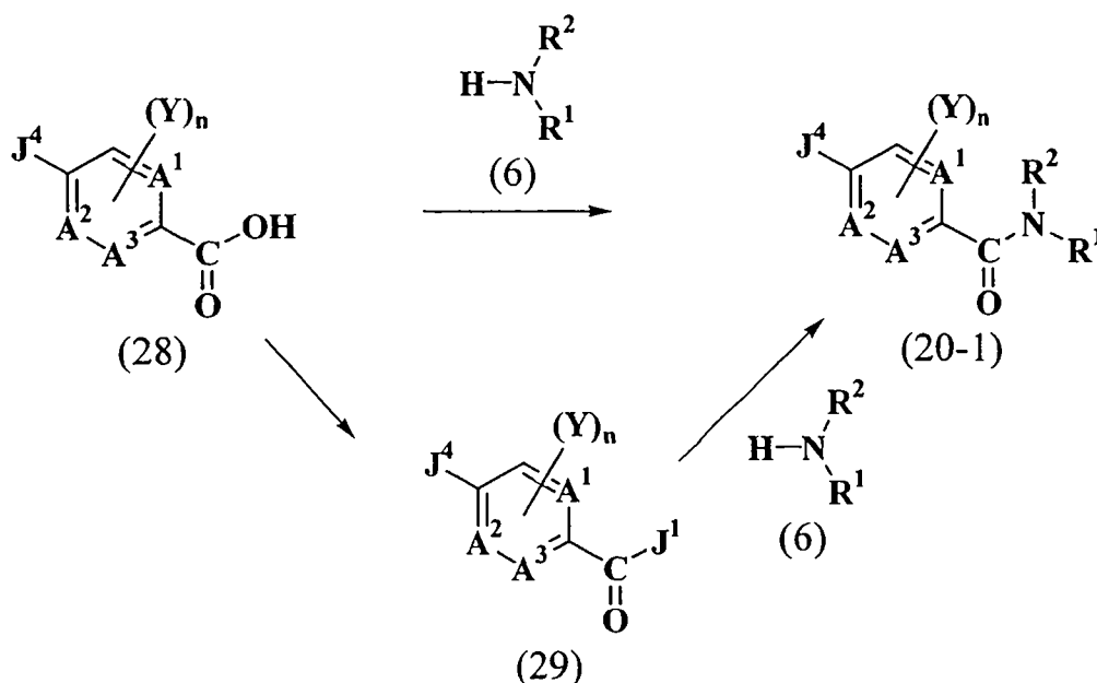
Reaction Scheme 8
