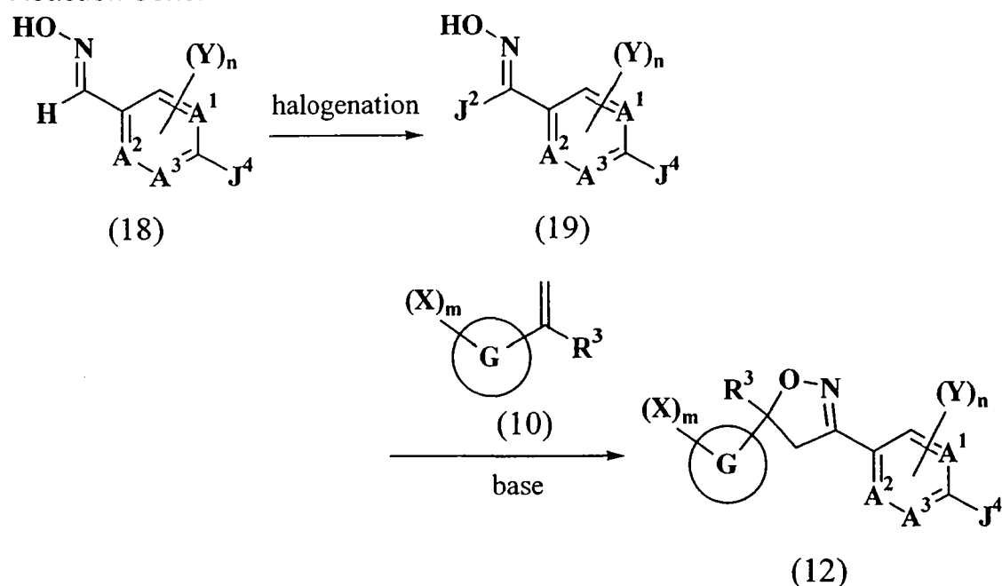
Reaction Scheme 4
