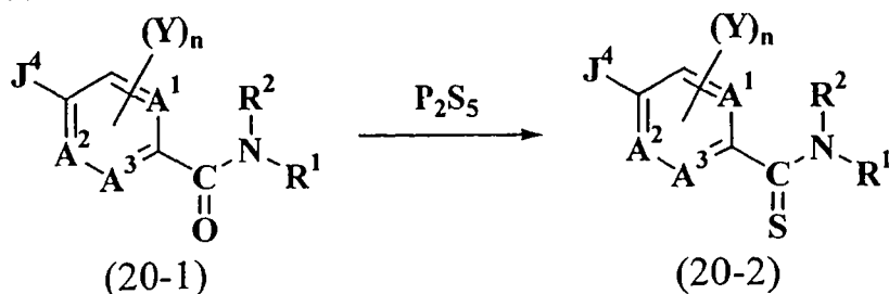
Reaction Scheme 9
