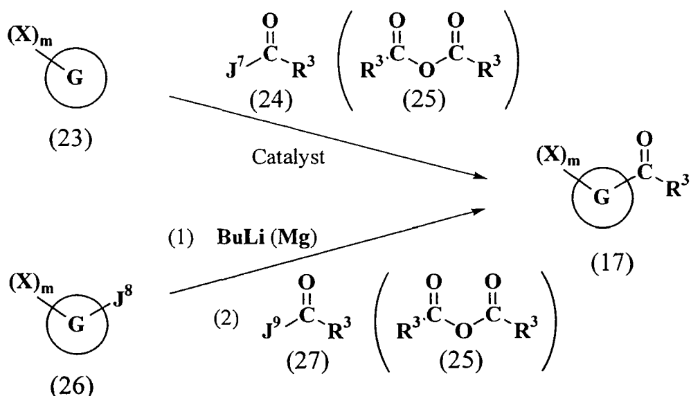
Reaction Scheme 7
