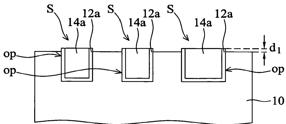
FIG. 4 (RELATED ART)
