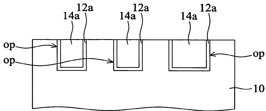
FIG. 3 (RELATED ART)
